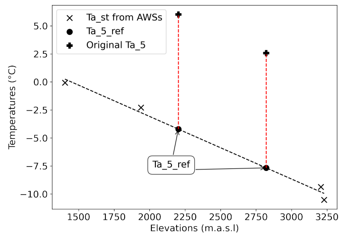
Figure 2. Example of Ta_{5\_ref} estimates for ERA5-Land grid elevations based on observed hourly ELR st (slope). The dashed black line represents the regression line of measured temperature to elevation. The red dashed lines show the difference of ERA5-Land Ta_5 to Ta_{5\_ref} (what it should be).
