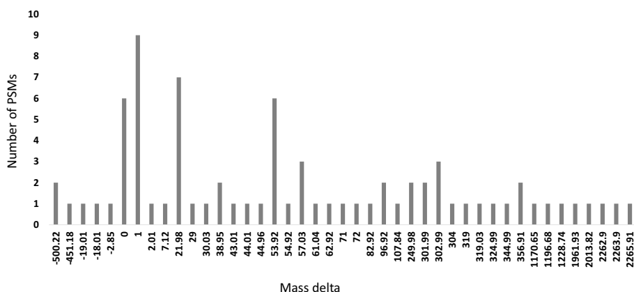
Fig. 5 Distribution of mass deltas carried by a set of spectra identifying peptide DATNVGDEGGFAPNIIENK. These spectra are interpreted from the file b1922_293T_proteinID_02A_QE3_122212
