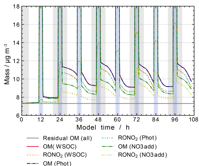
Figure 14. Processing of the organic mass fraction in the sensitivity runs investigating the influence of sink and source reactions for organic nitrates on aqueous-phase chemistry and composition. In addition to the scenario “WSOC”, rate constants of all NO 3 reactions with unsaturated organic compounds have been set to 10 7 M -1 s -1 in scenario “NO 3 add”, and photolysis reactions with j = 3.6 \times 10^{-7} s -1 have been added in scenario “Phot”. Cloud passages are shaded blue and night-time periods are shaded grey. Scenario names used in the legend are explained in Appendix A.2.
