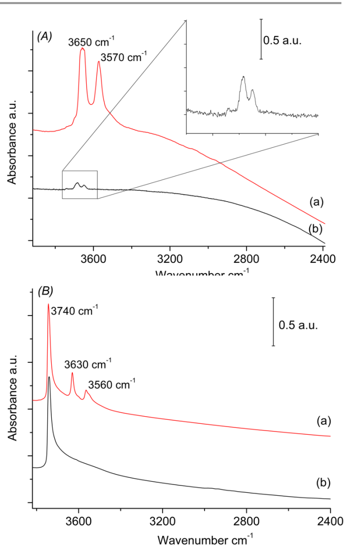
Figure 1. IR spectra after activation at 623 K and evacuation under secondary vacuum of zeolites X (A) and Y (B) in acidic (a) and sodium (b) forms.
