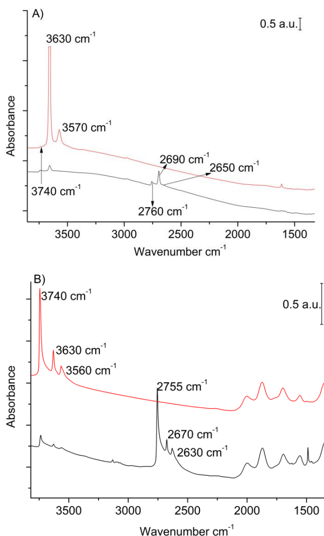
Figure 2. IR spectra after H/D isotopic exchange (black) and evacuation under secondary vacuum (red) at 573 K of zeolite X (A) and Y (B) in acidic forms.
