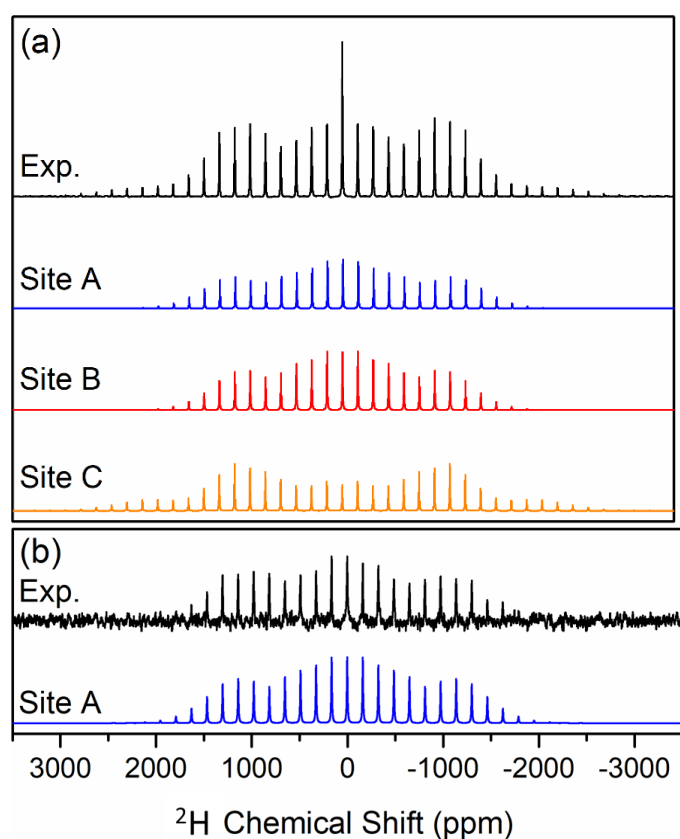
Figure 4. Experimental and corresponding fits of 2 H NMR spectra of deuterated 2 H-X (a) and Na-X (b). QUAD 1 st model was used from Dmfit software. For clarity, the intensity of sites A, B and C for deuterated 2 H-X zeolite sample are multiplied by 2, 2 and 200, respectively. The deconvoluted central spinning sidebands are presented in the SI (Figure S10).
