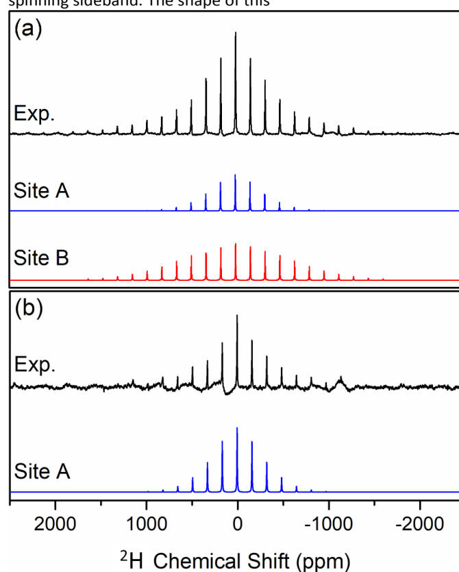
Figure 3. Experimental and corresponding fits of ^2\text{H} NMR spectra of deuterated H-Y (a) and Na-Y (b). 'Czjzek all' model was used from Dmfit software. The deconvoluted central spinning sidebands are presented in the SI (Figure S9).
