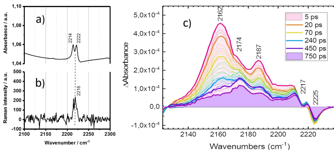
Figure 4: a) FTIR b) Raman and c) time-resolved IR spectra ( \lambda_{\text{pump}} = 420 \text{ nm} ) of DCA@ZSM-5 recorded in the region of the CN stretching mode.
