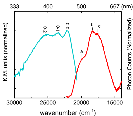
Fig. 2: Absorption in Kubelka-Monk unit, and emission spectra ( \lambda_{\text{exc}} = 420 \text{ nm} ) and DCA@ZSM-5
