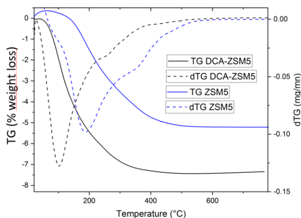
Fig. 1. TG (full line) and dTG (dash line) curves of ZSM-5 (blue) and DCA@ZSM-5 (black)
