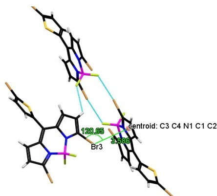
Figure 7. Br... \pi interaction ( d(\text{C9Br3}\cdots\pi \text{ centroid}) 3.586 Å, \angle(\text{C9}\text{--}\text{Br3}\cdots\pi \text{ centroid}) 120.65°) in BODIPY 3.
