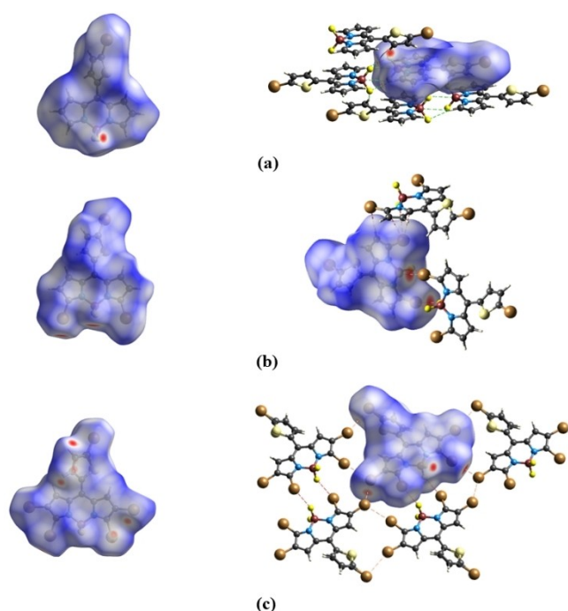
Figure 9. Hirshfeld surfaces (left) and related relevant supramolecular contacts involving halogen atoms (right) for 2 (a), 3 (b) and 4 (c).
