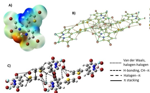
Figure 13. Results of the DFT and the QTAIM computational studies for BODIPY 4 , where A) is the ESP map, B) the MultiWFN visualization of the calculated non-covalent critical points and ring critical points and C) is a schematic representation of the intermolecular contacts directing the crystal packing of 4 .
