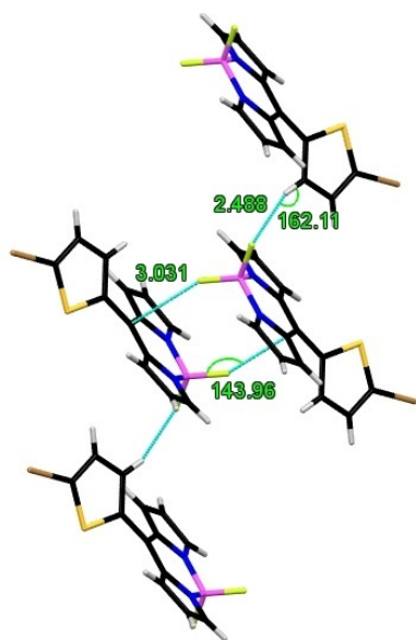
Figure 4. Crystal packing of BODIPY 2 and B-F2... \pi ( d(\text{F2}\cdots\text{C5}) 3.031 Å, \angle(\text{B-F2}\cdots\text{C5}) 143.96°) and C11-H11...F1 ( d(\text{H11}\cdots\text{F1}) 2.488 Å, \angle(\text{C11-H11}\cdots\text{F1}) 162.11°) interactions.
