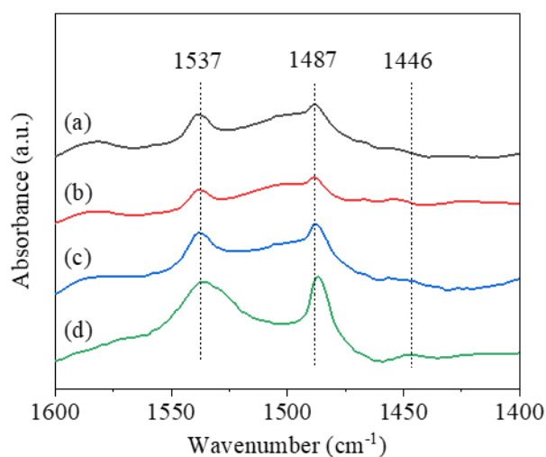
Figure 10. DRIFTS spectra of pyridine adsorbed on samples (a) MoVBiO-M-120, (b) MoVBiO-N-120, (c) MoVBiO-T-120 and (d) MoVBiO-T-175.
