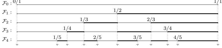
FIGURE 2. The Farey sequence of partitions
