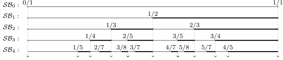
FIGURE 1. The Stern-Brocot sequence of partitions
