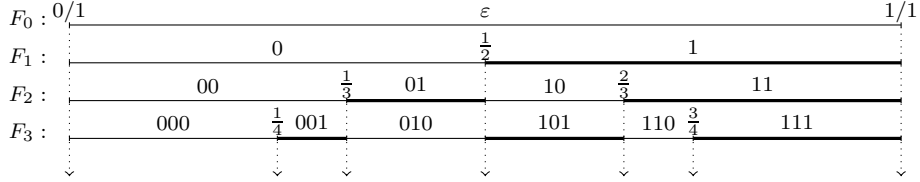
FIGURE 3. The labelling of the Farey partition F_n for n \leq 3 .
