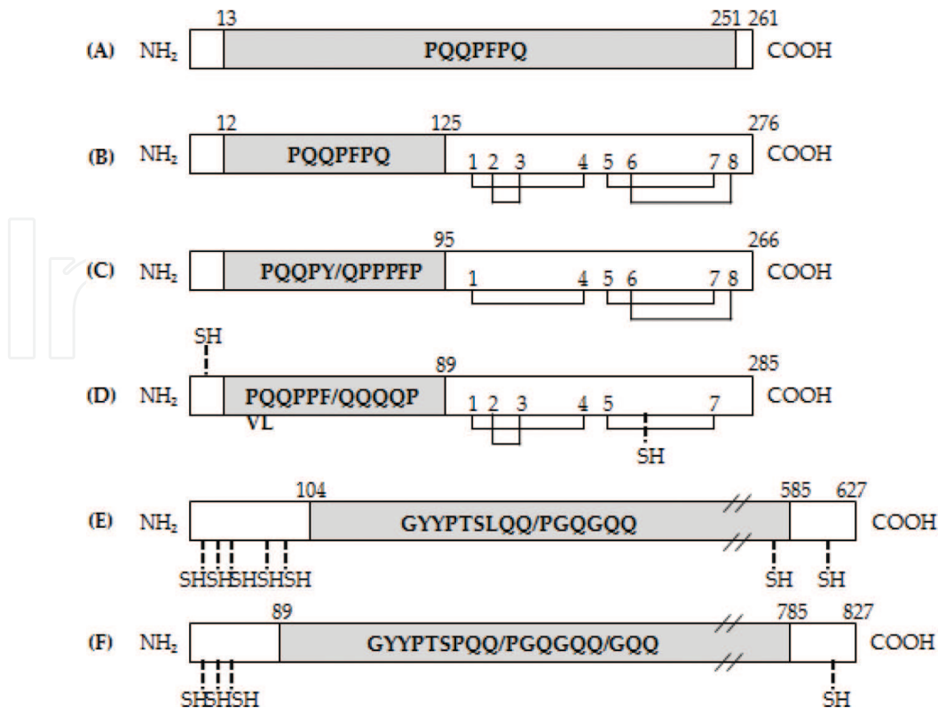
Figure 3. Schematic structures of typical primary structures of (A) \omega -gliadin, (B) \alpha -gliadin, (C) \gamma -gliadin, (D) LMW-GS, (E) HMW-GS \gamma and (F) HMW-GS x [15, 16]. Repetitive sequences are shaded and disulphide bonds between conserved cysteine residues (1–8) in the \gamma -gliadin are shown as lines. SH denotes the positions of cysteine residues in the HMW prolamins. Single letter abbreviations for amino acids: F = phenylalanine; G = glycine; L = leucine; P = proline; Q = glutamine; S = serine; V = valine and Y = tyrosine.
