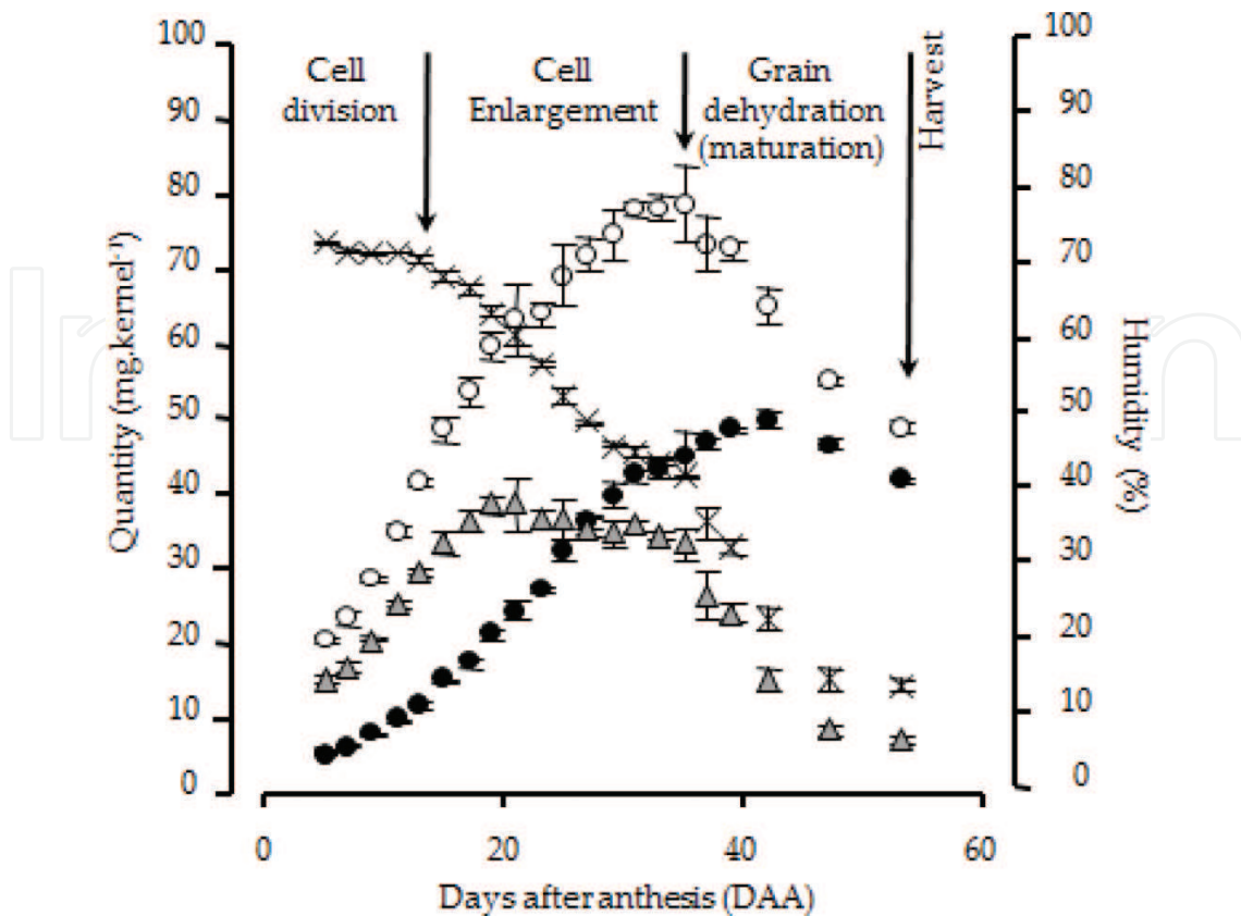
Figure 7. Grain filling period for a common wheat cultivar ( Soissons ). Evolution of (●) dry matter per kernel, (○) fresh matter per kernel, (△) water quantity per kernel and (×) grain humidity. The vertical lines represent the standard deviation ( n = 3 ) (from Carceller and Aussenac [67]).
