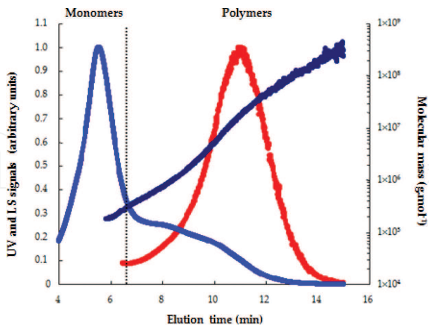
Figure 5. Asymmetrical flow field-flow fractionation (A4F) profiles of total solubilized storage proteins of a common French wheat cultivar (Soissons). UV (blue line), light scattering at 90^\circ (red line) and molecular weight in relation to elution time (dark line) (from Lemelin et al. [57]).
