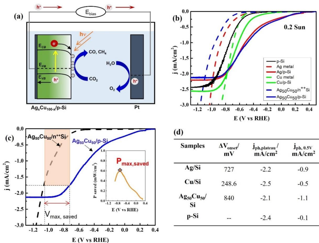
Figure 7: (a) Scheme of the PEC- \text{CO}_2\text{RR} using \text{Ag}_x\text{Cu}_{100-x} as photocathode and Pt as anode. (b) Polarization curves of p-Si, Ag/p-Si, Cu/p-Si and \text{Ag}_{50}\text{Cu}_{50}/\text{p-Si} under 0.2 sun illumination in \text{CO}_2 saturated 0.5 \text{ mol L}^{-1} \text{ NaHCO}_3 , and the corresponding dark electrodes. (c) Blue and black curves: polarization curves of \text{Ag}_{50}\text{Cu}_{50}/\text{p-Si} and \text{Ag}_{50}\text{Cu}_{50}/\text{n}^{++}\text{Si} (same conditions than in Fig 7b). Inset: power saved (calculated from Eqs. 5) vs. applied potential E for \text{Ag}_{50}\text{Cu}_{50}/\text{p-Si} (maximum at \diamond ). Orange rectangle: actual power saved at j/E corresponding to P_{\text{max,saved}} . At this point, V_{\text{max,saved}} = -0.69 \text{ V} and j = -1.67 \text{ mA/cm}^2 ; (d) \Delta V_{\text{onset}} ( = E_{\text{onset, photocathode}} - E_{\text{onset, dark electrode}} ), j_{ph} at the plateau and at 0.5 V_{\text{RHE}} (extracted from Fig. 7(b)). E_{\text{onset}} is chosen at j = -0.1 \text{ mA/cm}^2 .
