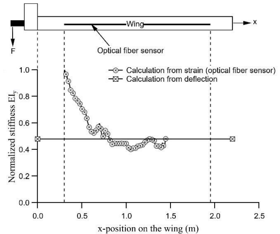
Figure 9. Wing stiffness
