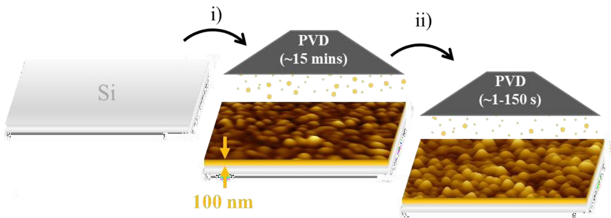
Scheme 1. Schematic representation of the fabrication of the SERS substrates. Two steps preparation method: (i) Deposit of 100 nm of gold by PVD on silicon wafer and (ii) additional gold depositions of increasing thickness (0 to 19.5 nm).
