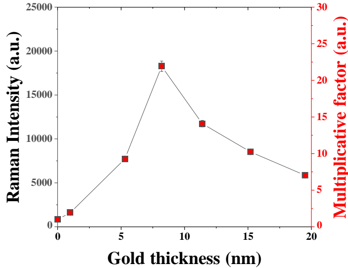
Figure 6. Average Raman intensity as function of the deposited gold layer thickness. The multiplication factors are calculated for each sample with respect to the reference (0s) Au substrate. P = 2 \text{ mW} ; t = 0.5\text{s} ; \lambda = 633 \text{ nm} .
