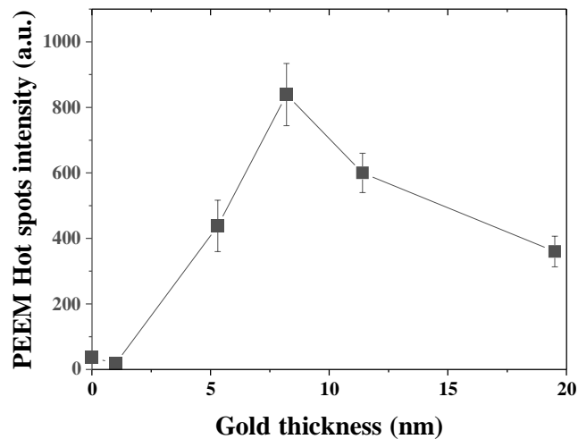
Figure 4. Averaged 3PPE PEEM Hot spot intensity per \mu\text{m}^2 as function of the thickness of the deposited gold layer. Laser wavelength \lambda = 633 nm, laser irradiance P = 2 \text{ GW}/\text{cm}^2 , P polarization under grazing incidence.
