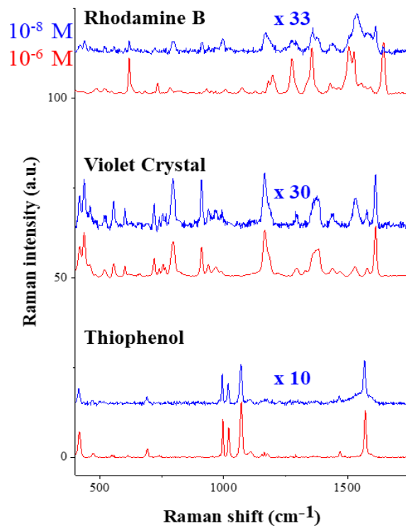
Figure 8. Averaged Raman spectra calculated from the recorded maps of rhodamine B, Violet Crystal and thiophenol at 10 -6 (red curve) and 10 -8 M (blue curve), respectively. P = 1 mW; t = 1; λ = 633 nm. The Raman spectra are vertically shifted and amplified by various factors (x33, x30 and x10) for clarity.
