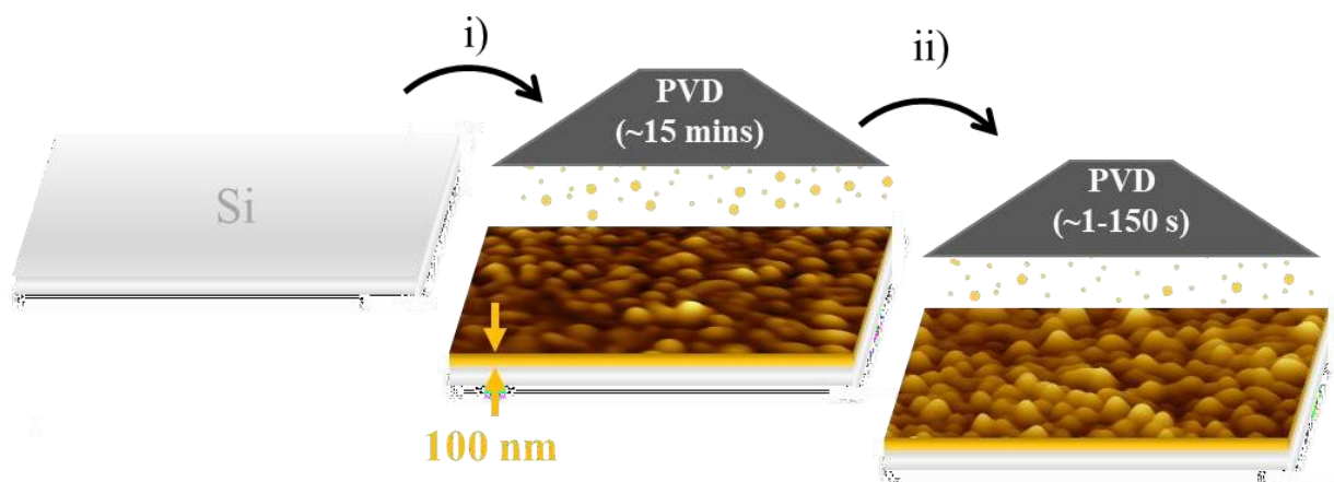
Scheme 1. Schematic representation of the fabrication of the SERS substrates. Two steps preparation method: (i) Deposit of 100 nm of gold by PVD on silicon wafer and (ii) additional gold depositions of increasing thickness (0 to 19.5 nm).
