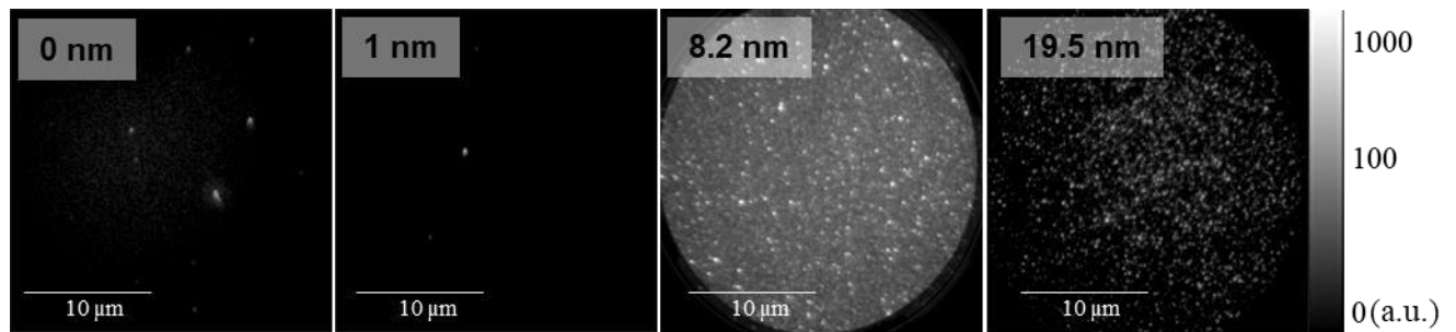
Figure 3. 3PPE PEEM images ( 25 \times 25 \mu\text{m}^2 ) of 0, 1.0, 8.2 and 19.5 nm gold layer deposited on 100 nm Au/Si substrate. PEEM intensities are normalized and displayed on a log scale. Laser wavelength \lambda = 633 nm, laser irradiance 2 \text{ GW}/\text{cm}^2 , p-polarization under grazing incidence, acquisition time t = 1 s.
