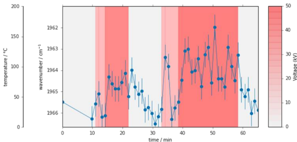
Figure 8: Wavenumber of the \text{BaSO}_4 band used to probe the \text{Ru}/\text{SiO}_2/\text{BaSO}_4 temperature in a \text{CO}_2/\text{CH}_4/\text{Ar} DBD plasma as a function of time. The intensity of the background color is indicative of the applied voltage, going from grey (0 kV, plasma off) to dark red (50 kV)
