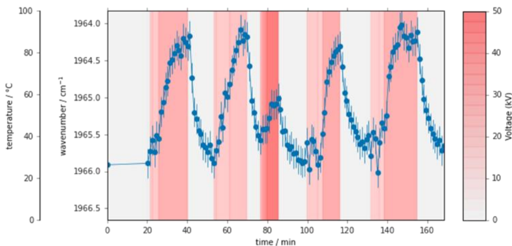
Figure 7: Wavenumber of the \text{BaSO}_4 band used to probe the \text{BaSO}_4 temperature in a \text{H}_2/\text{Ar} DBD plasma as a function of time. The intensity of the background color is indicative of the applied voltage, going from grey (0 kV, plasma off) to dark red (50 kV)
