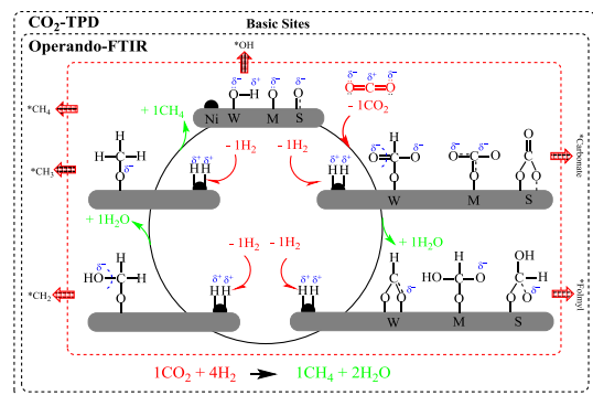
Figure 15. Proposed mechanism of \text{CO}_2 methanation over 3P-NMA
