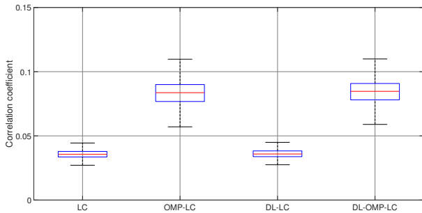
Figure 8: The output noise levels of LC, OMP-LC and DL-LC
