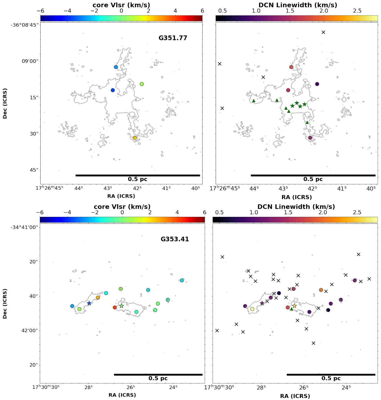
Fig. G.1. Core V_{LSR} (left) and DCN (3-2) linewidths (right) estimated from the DCN (3-2) fits to the continuum cores towards the intermediate protoclusters G351.77 (top) and G353.41 (bottom), respectively. The core V_{LSR} is the centroid velocity of the DCN (3-2) fit minus the cloud V_{LSR} (taken as -3 \text{ km s}^{-1} , and -17 \text{ km s}^{-1} for G351.77 and G353.41, respectively).
