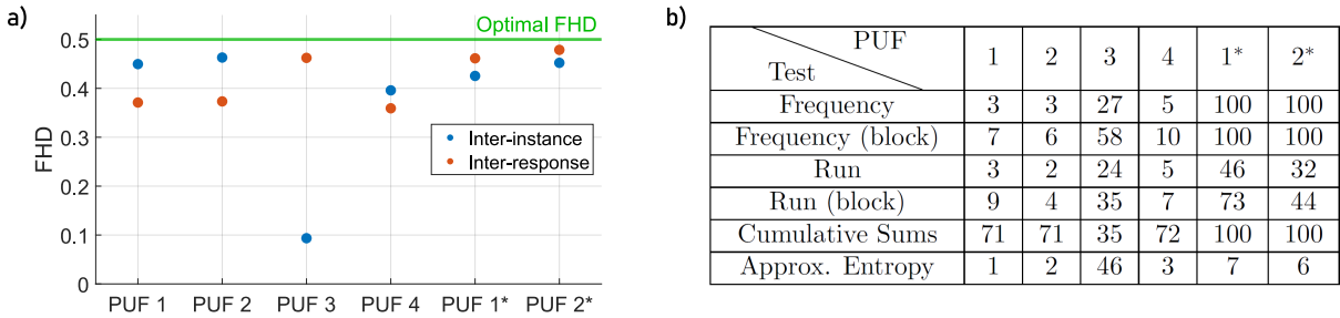
Fig. 2. a) Average inter-instance and average inter-response FHD of the different designs. b) Percentage of instances passing the considered NIST tests for each PUF design presented in Fig. 1 (b).
