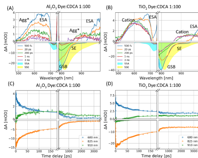
Figure 3. Transient absorption spectra of DSSCs prepared with \text{Al}_2\text{O}_3 (A) and \text{TiO}_2 (B) at different delay times. SSA: inverted steady-state absorption; SSE: inverted steady-state fluorescence. Kinetic traces are displayed at selected wavelengths for \text{Al}_2\text{O}_3 cell (C) and \text{TiO}_2 cell (D). The circles are the measured data points and the continuous lines are the fitted data. Excited state decay (680 & 825 nm) in the first 150 ps goes along with formation of the photoproducts (910 nm). Differences between \text{Al}_2\text{O}_3 and the \text{TiO}_2 cells can be found in the long-time behaviour: \text{Agg}^* decays but the cation absorption remains stable.
