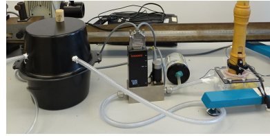
Figure 3. Picture of the player from left to right: pressure reservoir, flow controller, small reservoir, artificial mouth
