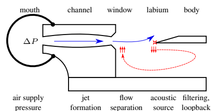
Figure 1. Schematic representation of the sound production mechanism in a recorder
