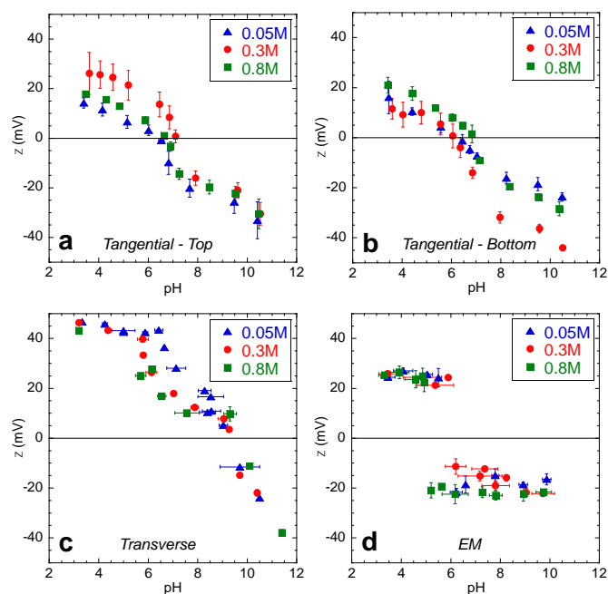
Figure 4. \zeta -potential evolution as a function of pH for OA-0.05 (blue triangles), OA-0.3 (red circles) and OA-0.8 (green squares) AAO membranes synthesized in oxalic acid solution at different concentrations measured by a ) tangential SC on top and b ) bottom surfaces, c ) by transverse SP and by d ) electrophoretic mobility (EM) of the grinded AAO membranes.
