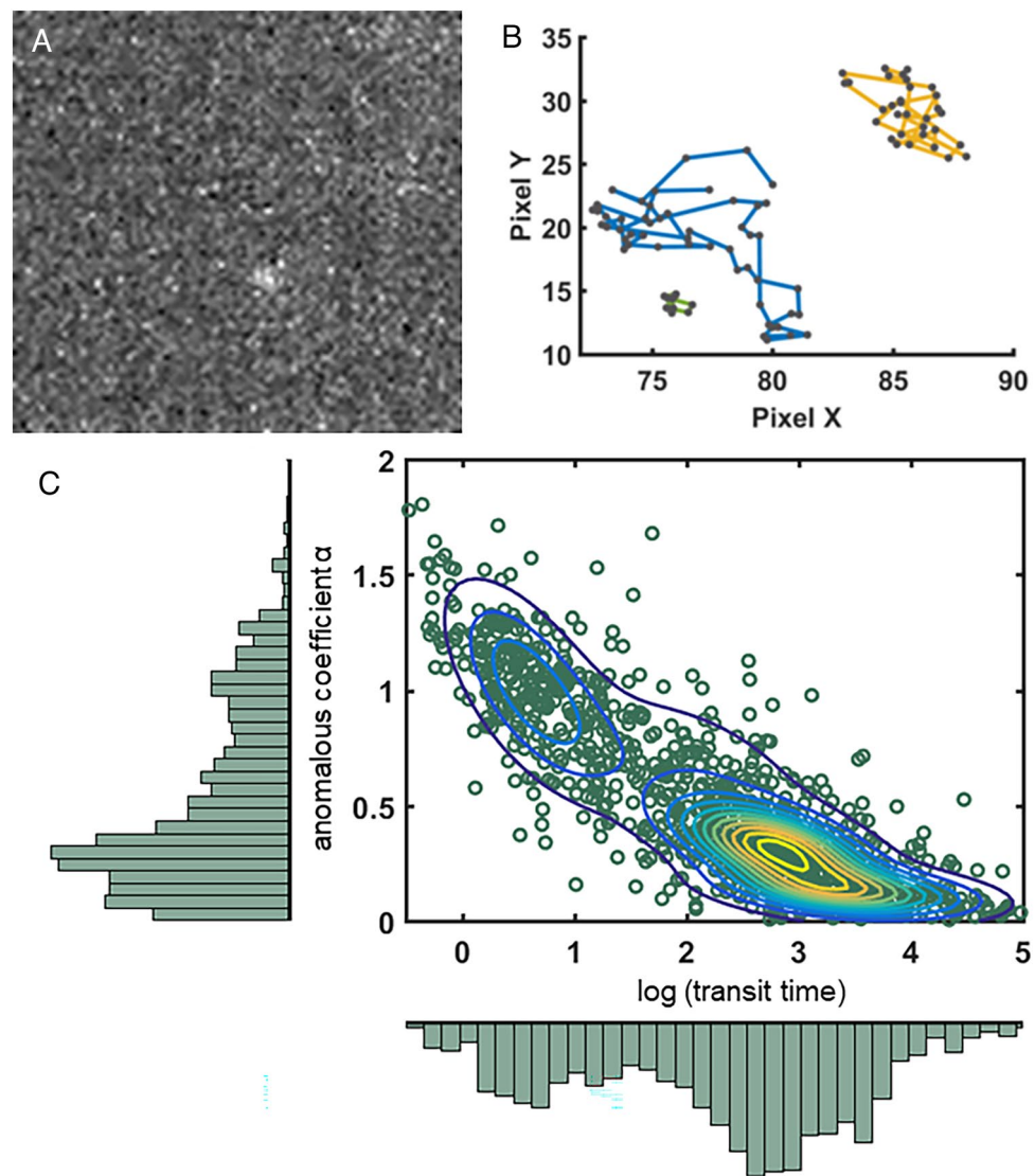
Figure 5. H-MSD SPT highlights the existence of distinct RPB1 subpopulations. (A) Picture representative of the signal-to-noise ratio obtained with JF549-halo tag at 0.1 nM in U2OS RPB1-Halo cells. (B) Examples of trajectory obtained with the tracking pipeline. (C) 1051 trajectories from SPT experiments carried out in the U2OS RPB1-Halo cell line ( n = 10 ), stained with JF549 at 0.1 nM, were analyzed by h-MSD. T_t and \alpha values from these experiments are represented in a scatter plot, in which concentric lines show the Probability Density Function given by the Gaussian Mixture Model. At least two distinct populations are clearly visible.
