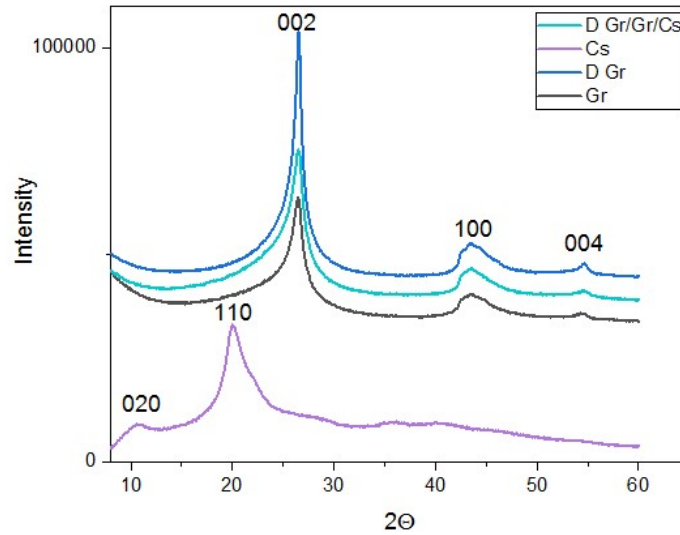
Figure 2: XRD patterns of the prepared ink (D Gr/Gr/Cs), chitosan, doped graphene (D.Gr) and Graphene (Gr).
