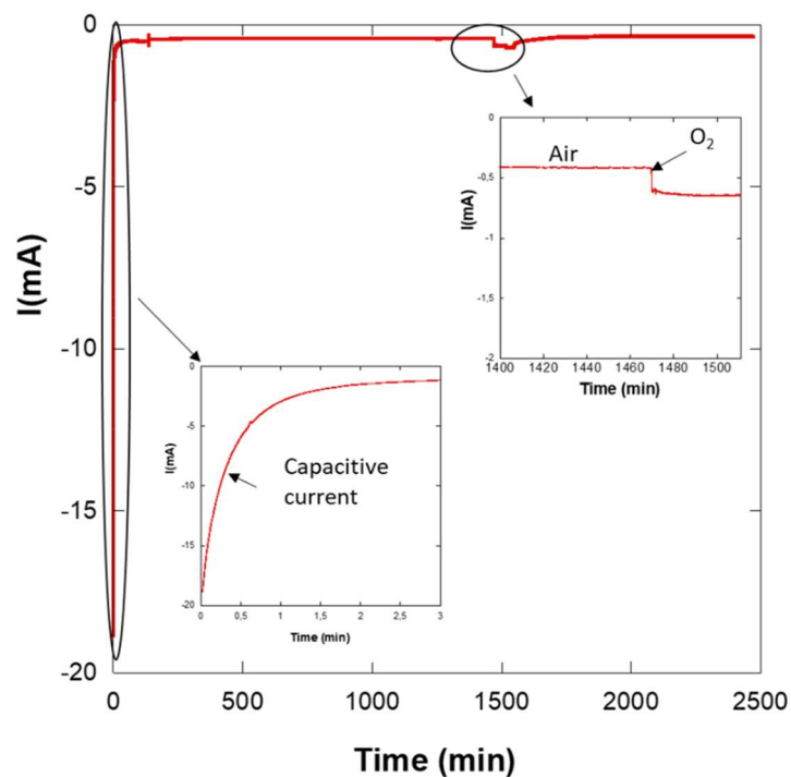
Figure 8: An example of chronoamperometry of sample 3 at 100 mV vs. SCE in 100 mL of a solution containing phosphate buffer (0.01 mol L -1 ), pH=7.4, and at ambient temperature (20 ± 3 °C).
