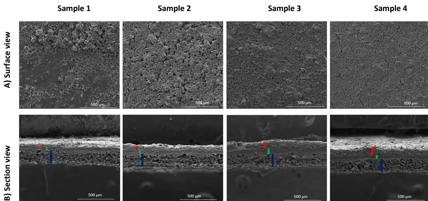
Figure 6: A) Surface views of the CNT-modified GDL and samples 1, 2, 3 and 4 B) Cross-section images of the coated CNT-modified GDL, and samples 1, 2, 3, and 4, where the red line for the coated layer, the green line for the GDL nano-porous layer (NPL) and the blue line for the GDL micro-porous layer (MPL).
