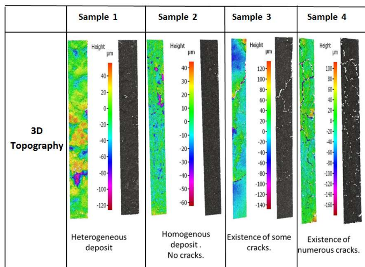
Figure 5: 3D topography images using Alicona for the four prepared samples.
