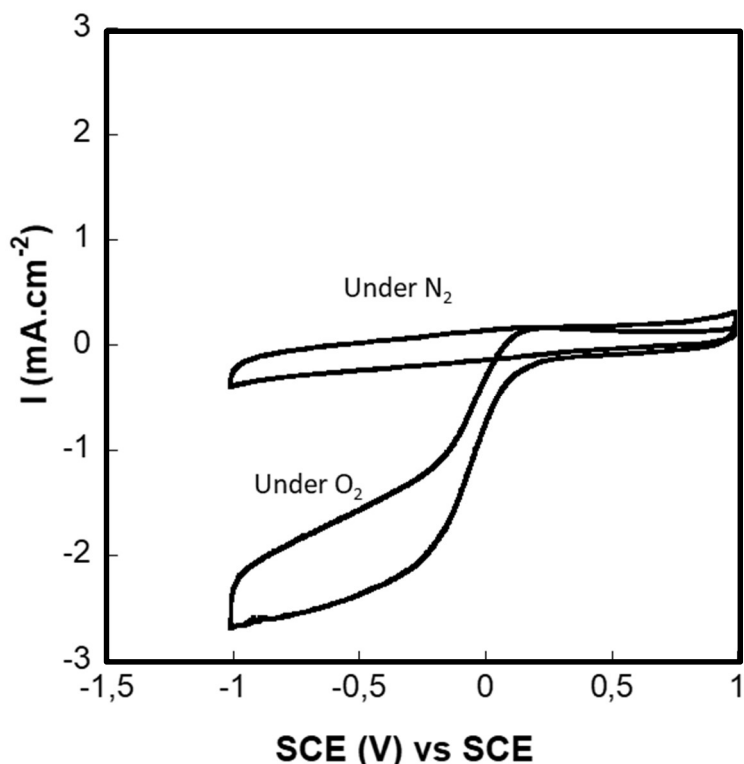
Figure 7: Cyclic voltammetry of the sample 2 ink diluted 10 times under air nitrogen and oxygen, in a PBS pH=7.4 at a scan rate of 10 \text{ mv.S}^{-1} and RDE speed of 500 rpm.
