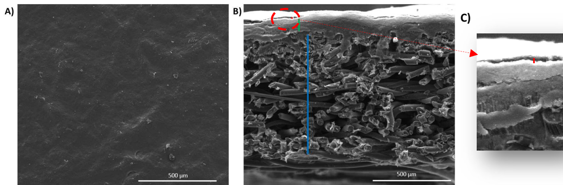
Figure 3: A) Surface views of the CNT-sprayed ink on the gas diffusion layer top (GDL) top. B) Cross-section images of the CNT-sprayed gas diffusion layer (GDL), where the red line for the sprayed layer, the green line for the GDL nano-porous layer (NPL), and the blue line for the GDL micro-porous layer (MPL). C) Zoom from the image B) showing the sprayed nanotubes layer (designed with a red line).
