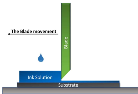
Figure 1: Schematic illustration of the Doctor blade printing working principle.
