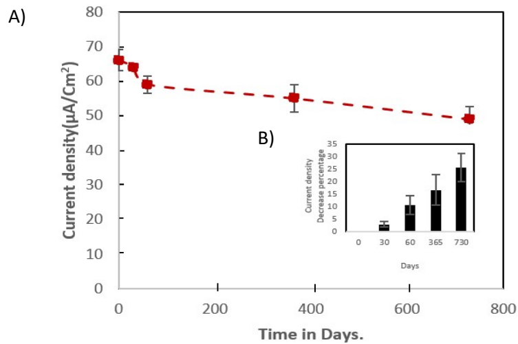
Figure 9: A) current density in the function of the time. B) Current density decrease percentage in the function of the time.
