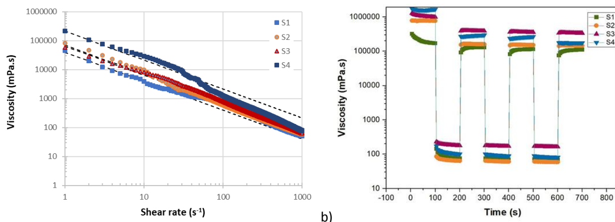
Fig. 2. a) Viscosity of MFC/chitosan/graphene hydrogels plotted as a function of the shear rate (dotted lines represent data interpolation with the Herschel-Bulkley law), b) the thixotropic behaviour of the different samples.
