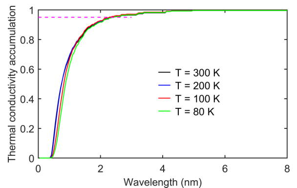
FIG. 8. Normalized thermal conductivity accumulation function versus phonon wavelength of bulk graphite along the basal-plane direction at different temperatures. The magenta dashed line denotes a 95% accumulation.
