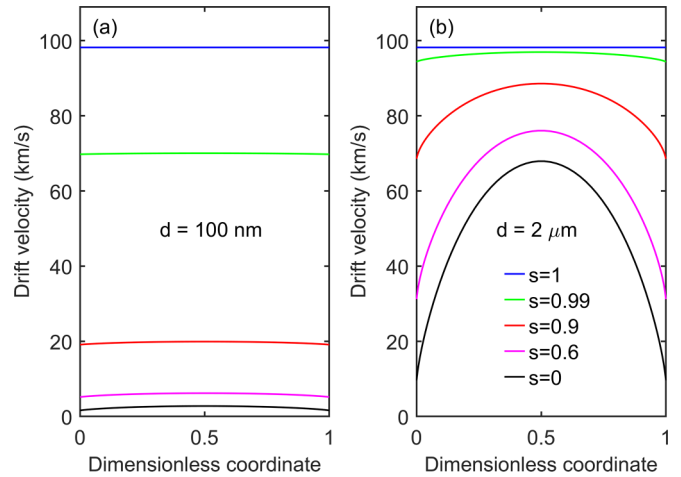
FIG. 5. Basal-plane phonon drift velocity distribution along the thickness direction in graphite thin film at 100 K and various surface specularity parameters ( s ): (a) thickness d = 100 nm; (b) thickness d = 2 \mu\text{m} . A temperature gradient of -1 \times 10^8 K/m is implemented.
