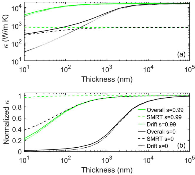
FIG. 4. Thermal conductivity decomposition in graphite thin film at 100 K: (a) thermal conductivity; (b) normalized thermal conductivity. The solid lines represent the overall result based on the phonon BTE under Callaway's dual relaxation model, whereas the dashed lines and dotted lines represent the single mode relaxation time (SMRT) part and drift correction. The normalization in (b) is done over the corresponding part in the bulk limit.
