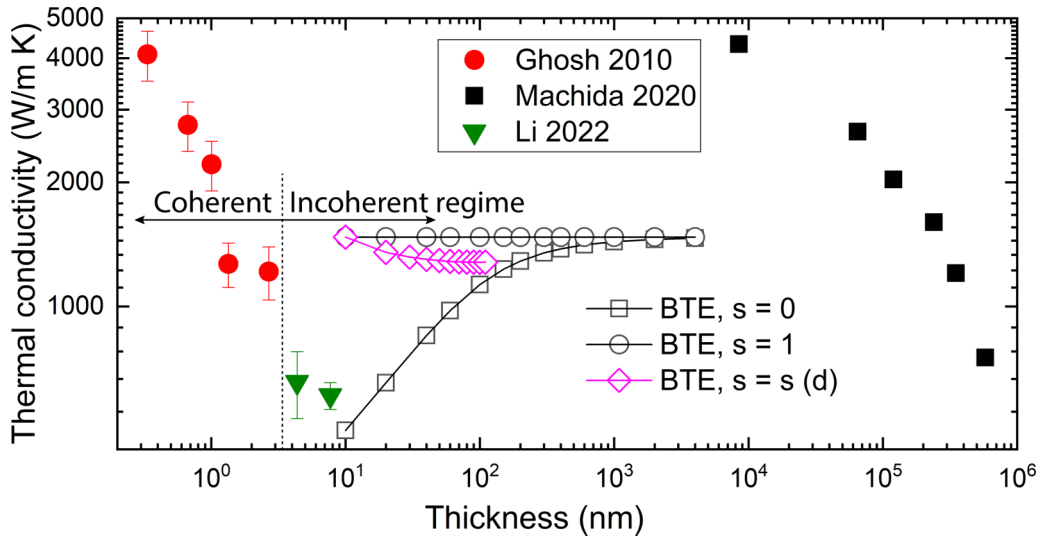
FIG. 7. Thickness-dependent thermal conductivity of graphite thin film along basal-plane direction around room temperature. The filled red circles denote the experimental data of multilayer graphene [17], the filled black squares denote the experimental data of graphite thin film at 250 K [20], and the filled green triangles denote the experimental data of 5.0 \mu\text{m} \times 3.4 \mu\text{m} \times 13 layers and 5.0 \mu\text{m} \times 3.7 \mu\text{m} \times 23 layers graphite samples [21]. The hollow black squares and circles with lines denote the present BTE model with a constant surface specularly parameter s = 0 and s = 1 , respectively. The hollow magenta diamonds with line denote the present BTE model with a specularly parameter ( s ) decreasing linearly from 1.0 to 0.5 as the thickness ( d ) increases from 10 to 110 nm [ s = s(d) ].
