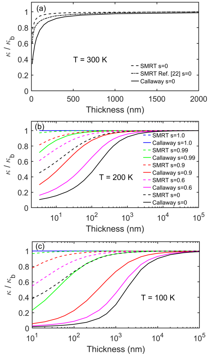
FIG. 3. Thickness-dependent normalized thermal conductivity of graphite thin film at different temperatures and various surface specularly parameters ( s ): (a) T = 300 K, natural graphite; (b) T = 200 K, isotopically pure graphite; (c) T = 100 K, isotopically pure graphite. The solid lines and dashed lines correspond to the present results based on phonon BTE under Callaway's dual relaxation model and under the single mode relaxation time (SMRT) model respectively. The dash-dotted line in (a) represents the reference SMRT model result [22]. In (a)–(c), \kappa_b = 1.4724 \times 10^3 , 3.1891 \times 10^3 , and 1.6688 \times 10^4 (W/m K), respectively, based on the present Callaway model, whereas \kappa_b = 472.9132 , 628.0705 , and 737.5010 (W/m K), respectively, based on the present SMRT model.
