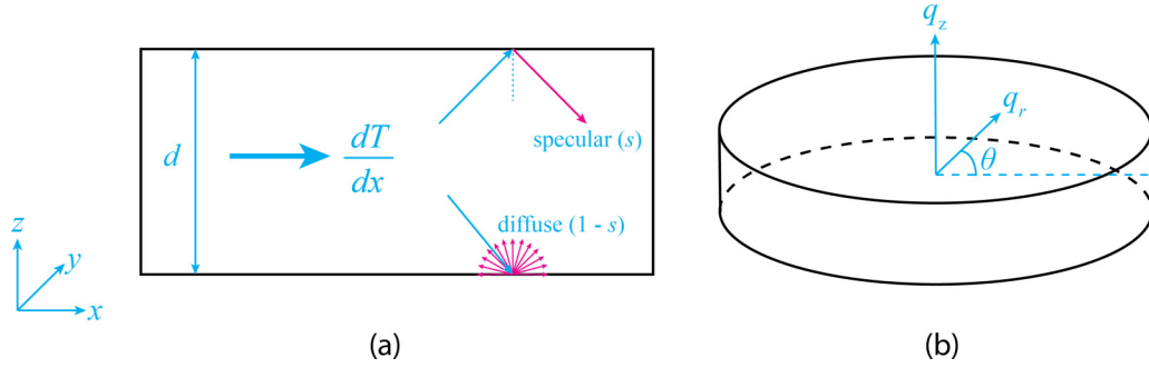
FIG. 1. Basal-plane phonon heat transport along a graphite thin film with a finite thickness d : (a) schematic of the physical model, where phonons experience partially specular and partially diffuse boundary scattering, with s referring to the specularly parameter; (b) approximate first Brillouin zone of graphite.
