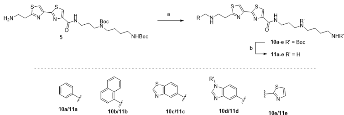
9 10 Scheme 4. Synthesis of the reductive amination series: compounds 11a-d . Reagents: a) 14a-d , AcOH, 11 NaBH 3 CN, MeOH, r.t.; b) HCl, MeOH, r.t.
