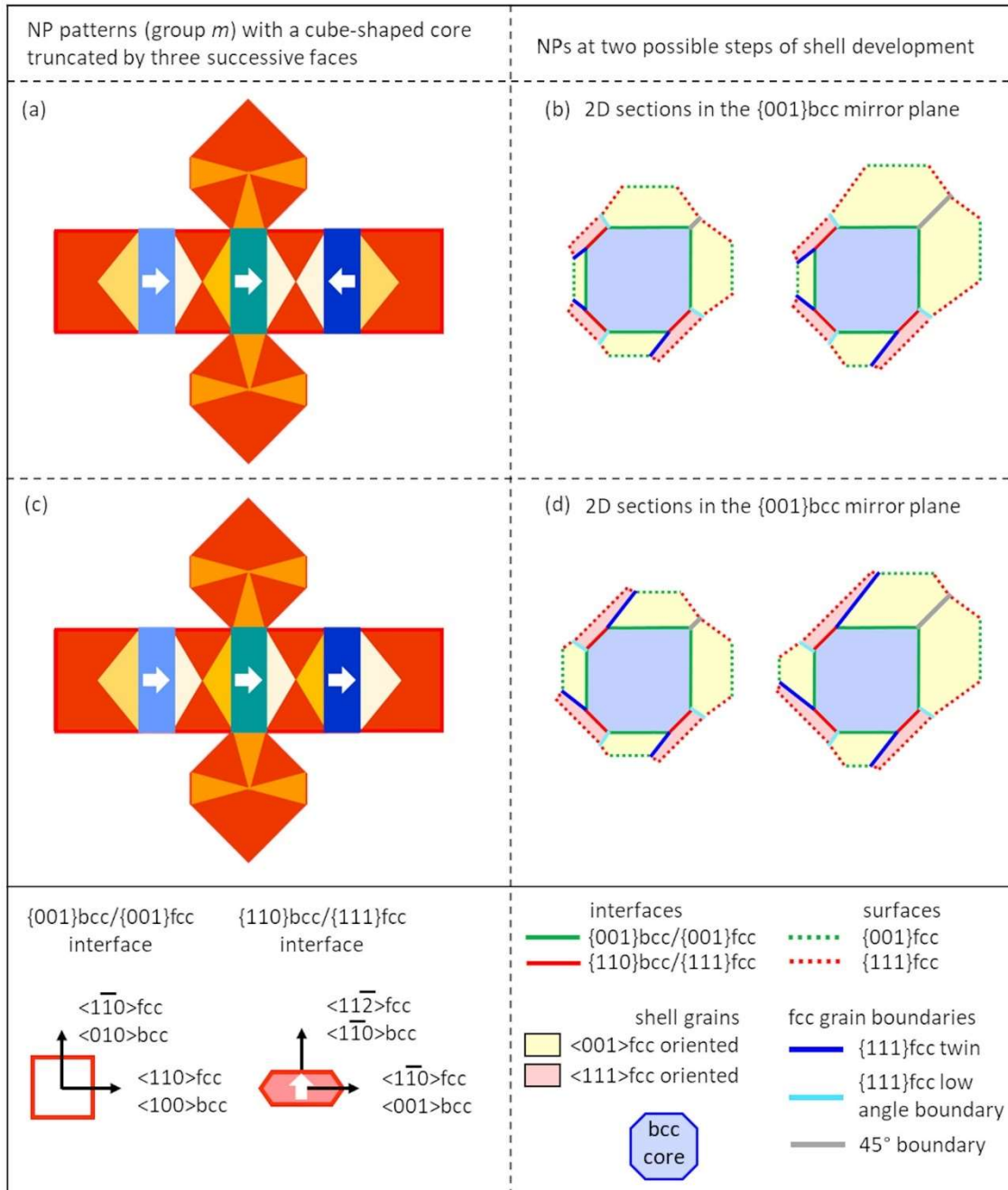
Fig.15 (a, c) Patterns of NPs with three truncations perpendicular to one \{001\} bcc plane. The white arrows symbolize the variants of \langle 111 \rangle_{\text{fcc}} oriented grains growing on the \{110\} bcc truncated faces. Light, medium or dark yellow shade indicate that the nearest neighbor of a \langle 001 \rangle_{\text{fcc}} oriented grain will be a \langle 111 \rangle_{\text{fcc}} oriented grain separated by a twin boundary, a LAGB boundary or the third type of boundary, respectively, and chestnut color indicates that the neighbor will be another \langle 001 \rangle_{\text{fcc}} grain separated by a 45^\circ boundary. (b, d) 2D sections in the mirror plane at different possible stages of the shell evolution.
