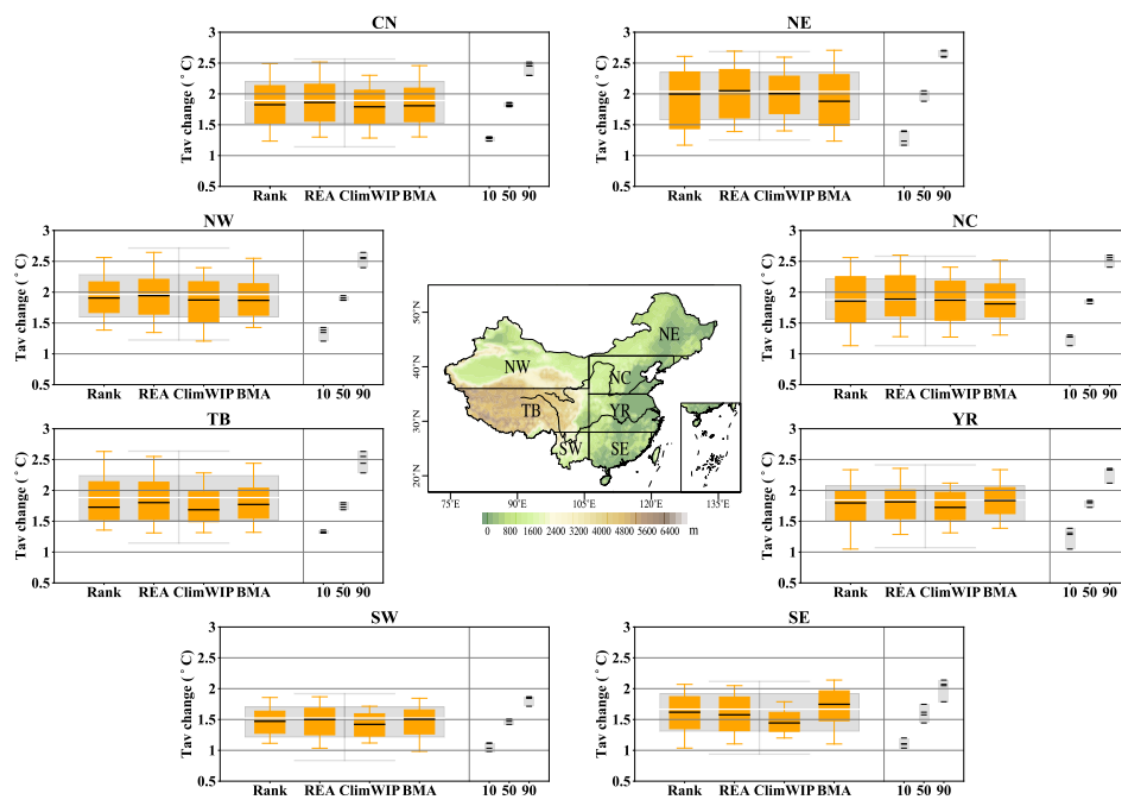
Fig. S1. As in Fig. 3., but for the changes under 2 ^{\circ}\text{C} global warming target.
