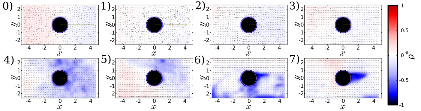
Fig. 18 Multiparticle model: density and velocity, for the 8 cases outlined in Tables 10 and 11.
