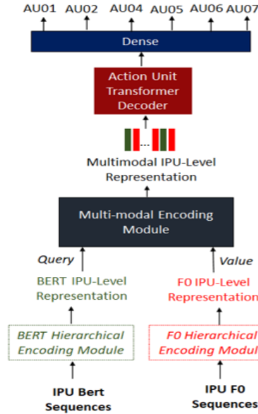
Fig. 1. "I-Brow" overall architecture. The network takes as input sequences of fundamental frequencies that correspond to one Inter-Pausal Unit (IPU) - sequence of continuous stretch of speech in one speaker's channel, delimited by a silence of more than 200ms -, and the corresponding text bert embeddings. With its hierarchical property, it encodes the input features at both word-level, and IPU-level, then generates a multimodal IPU-level representation of the input features. The network then learns to map the resulting representation to upper-facial - eyebrows - gestures.
