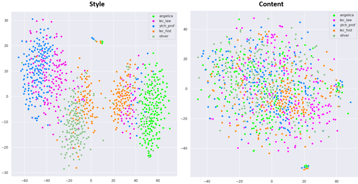
Figure 5: Left: T-SNE visualization of the style embeddings on the test sets of 5 speakers. Right: T-SNE visualization of the content embeddings on the same test sets.
