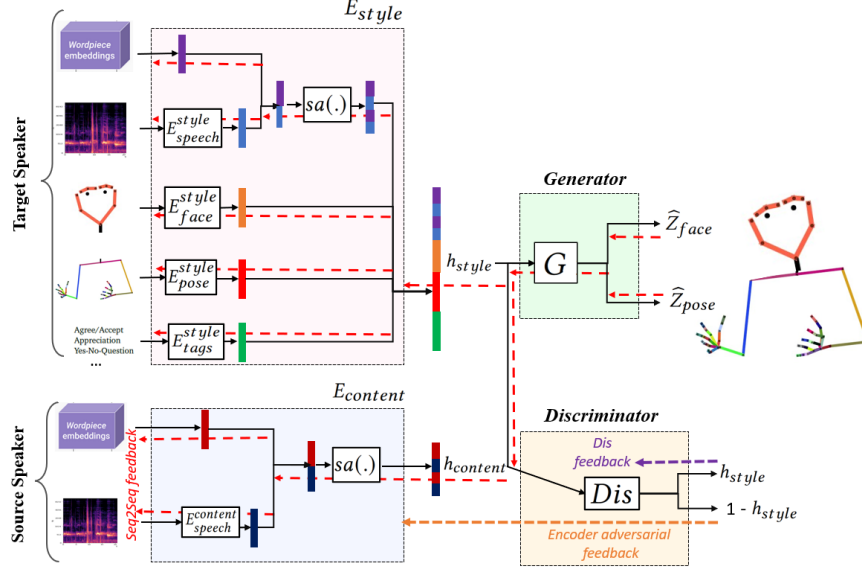
Figure 1: Overview of TranSTYler , an approach driven by the content of a source speaker’s speech - text semantics ( X_{text}^{source} ) and Mel spectrogram ( X_{speech}^{source} ) - and conditioned on a target speaker’s style vector h_{style} generated from the target’s multimodal input data - Mel spectrogram ( X_{speech}^{target} ), 2D facial landmarks ( X_{face}^{target} ), 2D poses ( X_{pose}^{target} ), and dialog tags ( X_{tags}^{target} ). The network is composed of: (1) a style encoder that encodes the target’s multimodal data and generates the style vector h_{style} , (2) a content encoder that encodes the source’s speech content and generates the content vector h_{content} , and (3) a discriminator Dis used during training time to disentangle h_{content} and h_{style} . A generator G is used to generate body \hat{Z}_{pose} and facial \hat{Z}_{face} gestures.
