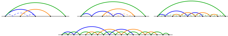
■ Figure 10 An iterated subdivision. Created edges have the color of the edge they stem from.
