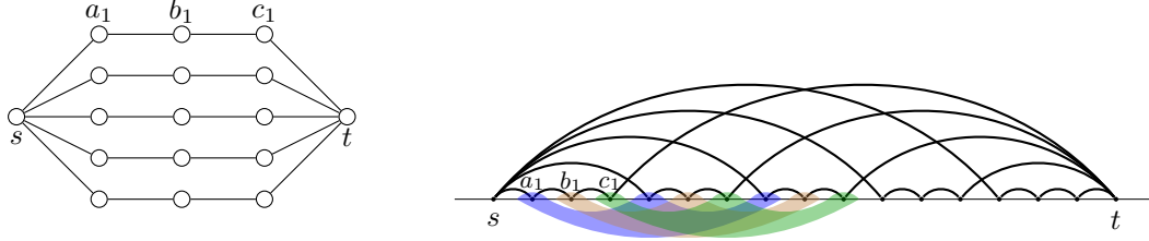
■ Figure 2 Left: The graph H_5 . Right: The same graph drawn along an orderable (together with an appropriate sequence) to witness low stretch-width. The parts A, B, C maintained by the partition sequence are depicted in blue, brown, green, after the iteration i = 3 .
