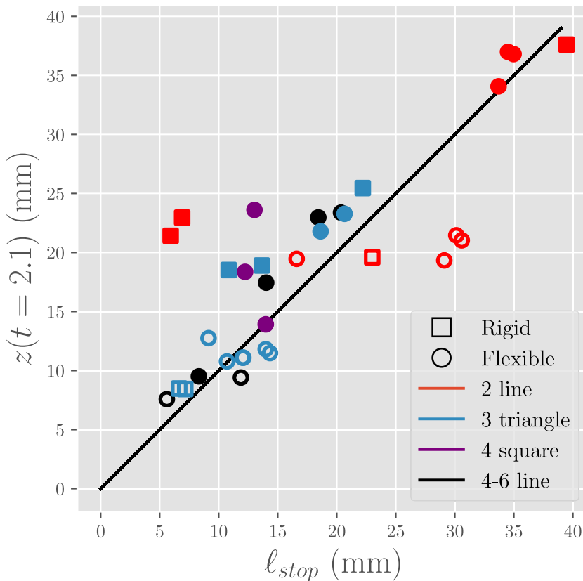
FIG. 5. Comparison between predicted and measured penetration length for a wide variety of fiber arrays with \Phi = 2.76 . Open symbols are for 0.25 ml drops and filled symbols are for drops with 0.25 \text{ ml} < \text{volume} \leq 1.0 \text{ ml} .
