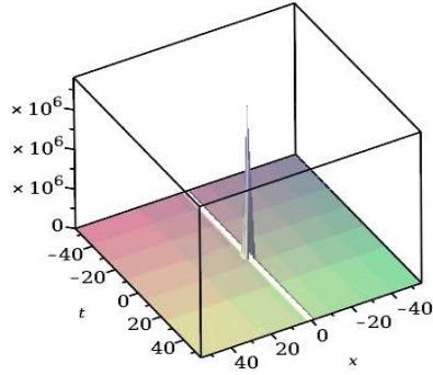
Figure 9. Solution of order 9 to (1).
