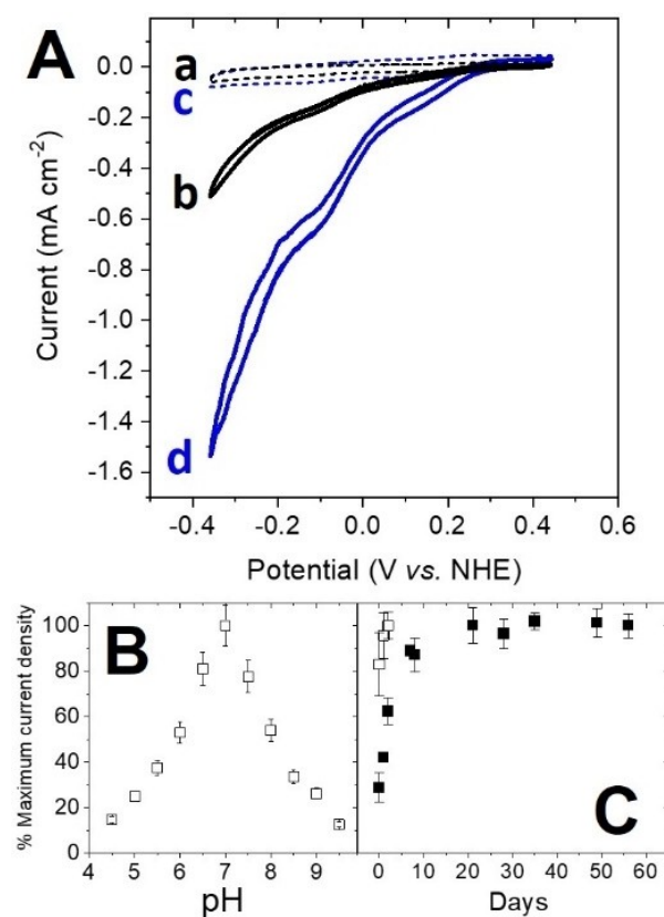
Figure 2. (A) CV of A. faecalis NiR-functionalized electrodes (a) before and (b) after addition of 20 mM \text{NaNO}_2 for pristine MWCNT electrodes, and (c) before and (d) after addition of 20 mM \text{NaNO}_2 for ADA MWCNT electrodes (50 mM Tris-HCl buffer pH 7.0, 30 mM \text{Na}_2\text{SO}_4 ; v = 5 \text{ mV s}^{-1} ). (B) Percentage of maximum electrocatalytic activity against pH values; (C) Plot of the percentage of maximum electrocatalytic activity over time. Filled black squares (■) represent the electrodes used directly after NiR immobilisation on MWCNTs and stored in 50 mM Tris-HCl buffer pH 7.0, 10 mM \text{NaNO}_2 at 21 °C under Ar atmosphere. Empty black squares (□) represent the electrodes pre-activated by chronoamperometry at the potential of -0.4 \text{ V} vs. NHE in presence of 20 mM \text{NaNO}_2 (50 mM Tris-HCl buffer pH 7.0, 30 mM \text{Na}_2\text{SO}_4 ).
