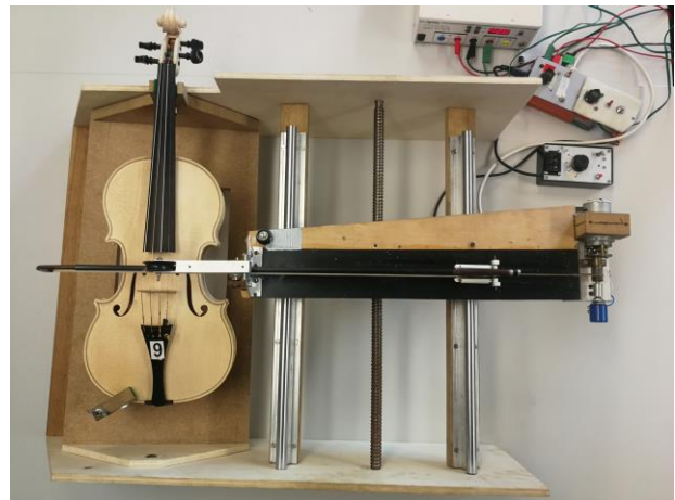
Figure 3. Bowing machine
