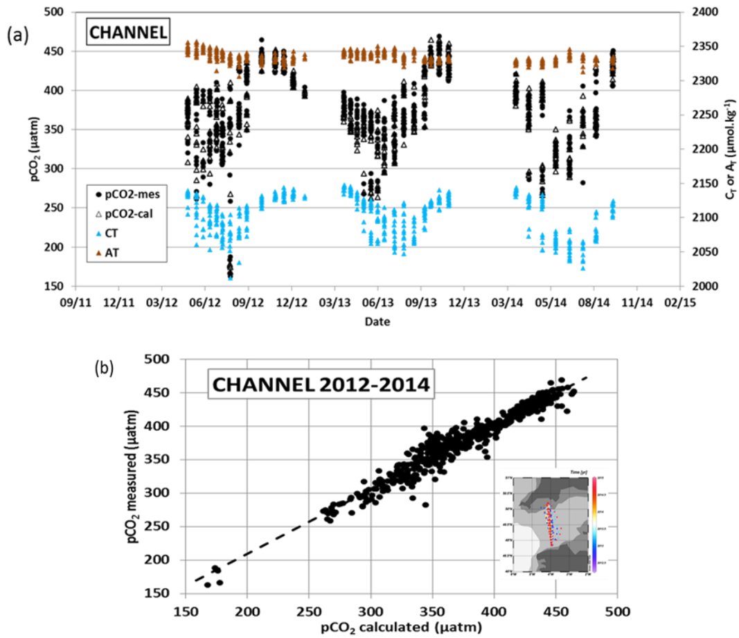
Figure 6: (a): Time-series of A_T (brown triangles, right Y-axis), C_T (blue triangles, right Y-axis), p\text{CO}_2 calculated (open triangles, left Y-axis) and p\text{CO}_2 measured (filled circles) in the Western English Channel in 2012-2014 (Marrec et al., 2014). (b): Measured p\text{CO}_2 versus calculated p\text{CO}_2 for the same samples. The mean difference ( p\text{CO}_{2\text{cal}}-p\text{CO}_{2\text{mes}} ) for 528 samples is -1.9 \mu\text{atm} ( \pm 11.9 \mu\text{atm} ). Data from Marrec and Bozec (2016 a,b; 2017). Localization of the samples is shown in the inserted map.
