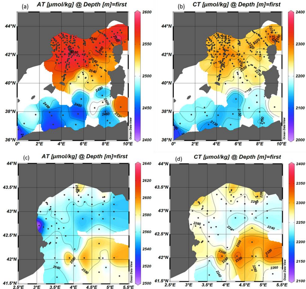
943 Figure 11: Distribution of A_T (a) and C_T (b) in \mu\text{mol kg}^{-1} in surface waters of the Western Mediterranean Sea (0- 944 10m) from all data for 1998-2019. Detailed distribution of A_T (c) and C_T (d) in \mu\text{mol kg}^{-1} in surface waters of the 945 Gulf of Lion for the period 2010-2011 only (cruises CARBORHONE, CASCADE, LATEX, MOLA, MOOSE- 946 GE). Figures produced with ODV (Schlitzer, 2018). 947
