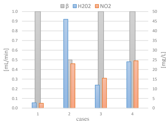
Graph 1. Generation rate (left axis) and concentration of \text{H}_2\text{O}_2 and \text{NO}_2^- (right axis) in PTW
