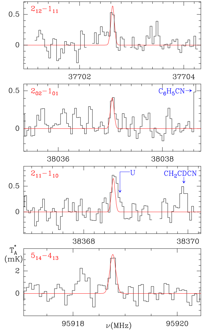
Fig. 2. Lines of H 2 CCCH + observed in the 31–115 GHz domain toward TMC-1. The abscissa corresponds to the rest frequency in MHz. The ordinate is the antenna temperature corrected for atmospheric and telescope losses in mK. The spectral resolution is 38 kHz below 50 GHz and 48 kHz above. The line parameters are given in Table B.1. The red lines show the computed synthetic spectra (see text).
