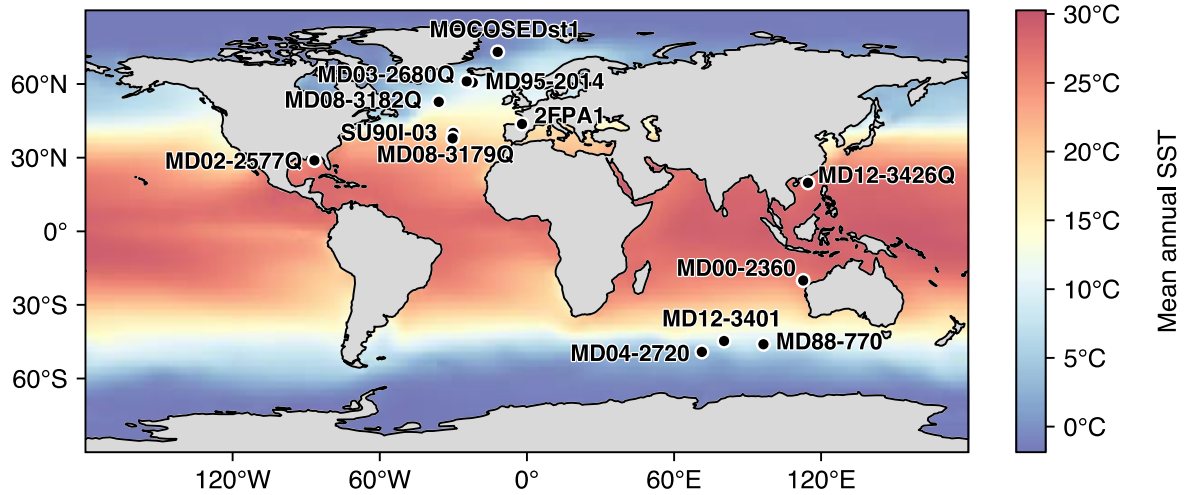
Figure 1: Map showing the location of core-tops used in this study, with the mean annual SST from WOA13
