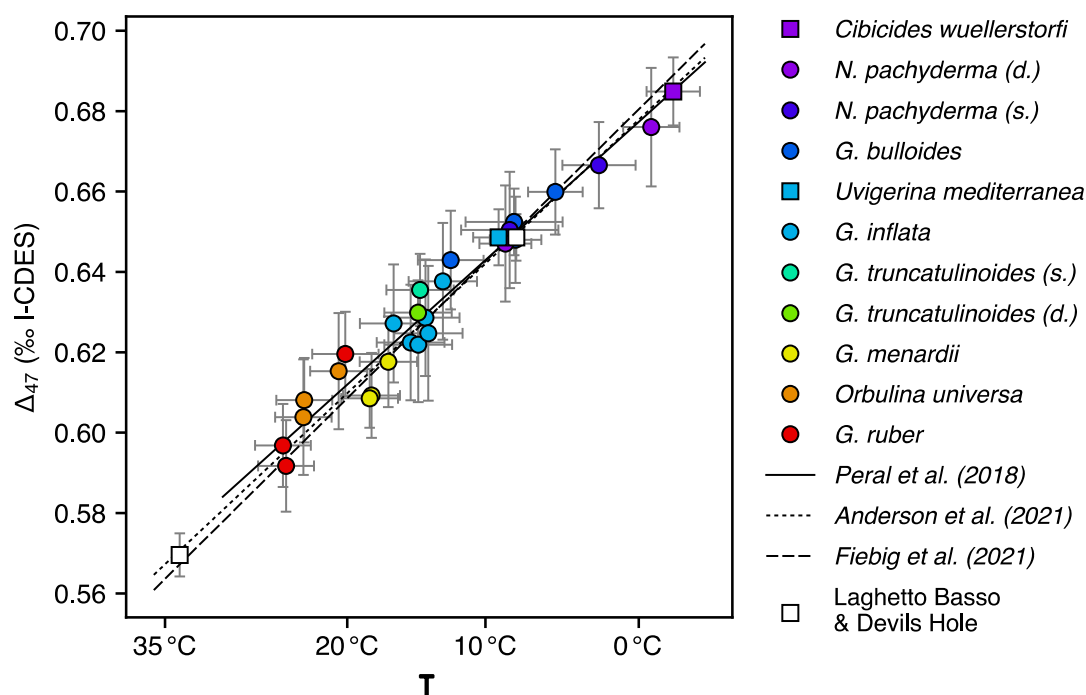
Figure 4: Recalculated \Delta_{47} values (mean and 2SE) compared to oxygen isotopic temperatures (mean and 2SE) obtained with Kim and O’Neil (1997) for planktonic (circle) and benthic (square) foraminifera samples, combining all size fractions (modified from Peral et al., 2018). The new calibration regression corresponds to the black line (Peral et al., 2018 recalculated). The recalculated foraminiferal calibration is compared to the slow-growing calcite from Laghetto Basso and Devils Hole (from Anderson et al., 2021) and to calibrations of Anderson et al. (2021) and Fiebig et al. (2021)
