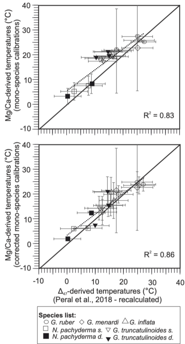
Figure 5: Mg/Ca-derived temperatures using mono-species calibrations, compared to the \Delta_{47} -derived temperatures using the recalculated Peral et al. (2018) calibration (a) and the Mg/Ca-derived temperatures using the corrected Mg/Ca mono-species calibrations for salinity and pH compared to the \Delta_{47} -derived temperatures using the recalculated Peral et al. (2018) calibration (b). The dotted linear regression, excluding O. universa and G. bulloides , is plotted. A line 1:1 is plotted in black; uncertainties are at 2 SE.
