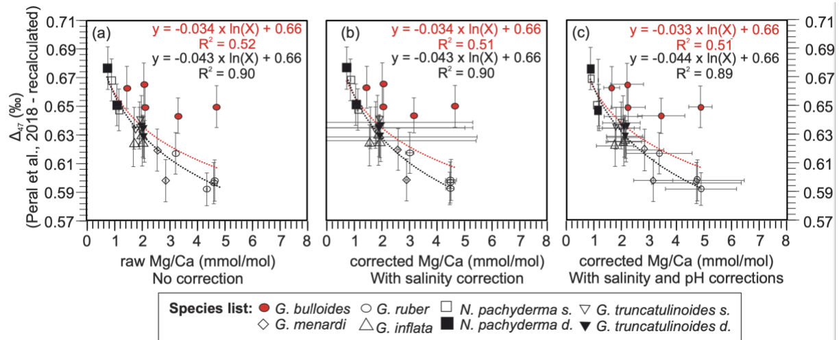
Figure 3: Comparison of our recalculated foraminiferal \Delta_{47} values with raw Mg/Ca values (uncorrected) (a), with corrected Mg/Ca for salinity only (b), and with corrected Mg/Ca for salinity and pH (c). The Mg/Ca values are corrected using the equations from Gray and Evans (2019), the salinity and pH from the atlas and the oxygen isotopic temperatures. The red dotted logarithmic regressions are plotted for all the plots, including G. bulloides and the black dotted regressions are without G. bulloides . All the uncertainties are at 2SE.
