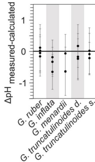
Figure 6: the difference for all the species from our dataset (excluding O. universa , G. bulloides and N. pachyderma ) between the extracted pH from the atlas (GLOPAD 2020) and the reconstructed pH, using the equations from Gray and Evans (2019) with the raw Mg/Ca, the \Delta_{47} -derived temperatures, and the combination of \delta^{18}\text{O} and \Delta_{47} -derived temperatures to reconstruct the \delta^{18}\text{O}_{\text{sw}} . The uncertainties correspond to the uncertainties associated with the reconstructed pH (2SE)
