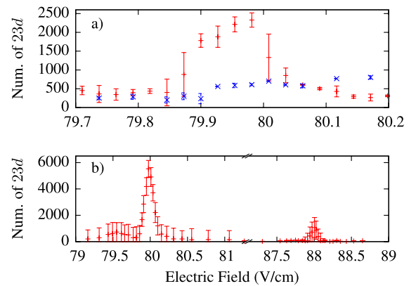
FIG. 4 (color online). Figure (a) shows the number of detected d atoms as a function of the applied electric field for exciting the p (red +) and s (blue \times ) states, with an s density comparable or greater in the s excitation than in the p excitation. The on-resonant 4-body process creates more than a factor of 4 more d atoms than the off-resonant s \rightarrow d 2-body process at 79.99 V/cm. Figure (b) shows the number of detected d atoms when exciting the p \rightarrow s resonance for the |m_j| = 1/2 (79.94 V/cm) and |m_j| = 3/2 (88.14 V/cm). We observe no significant d state population in the |m_j| = 3/2 case.
