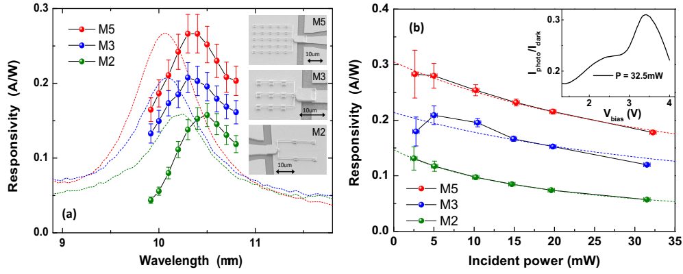
Fig. 1. (a) Room-temperature responsivity vs wavelength of the QWIPs studied in this work, measured with an extended-cavity QCL (dots). The incident power is of 4.3 mW. For comparison, the absorption spectrum of each device measured with an FTIR spectrometer, normalised to its peak responsivity is also reported (dashed lines). The devices are labelled respectively M5, M3 and M2, and their SEM pictures are shown on the right. For all of them the patches consist of metallic squares of lateral side s = 1.8 \mu\text{m} . In the M5 and M3 devices, individual patches are separated by a period p = 5 \mu\text{m} , while for device M2 we used p = 10 \mu\text{m} . As shown in the pictures, patches are electrically connected together and to a 50 \Omega integrated coplanar line by a suspended gold wires of \sim 150 \text{ nm} diameter (only the first part of the coplanar line is visible in the SEM images). (b) Responsivity vs incident power at \lambda = 10.3 \mu\text{m} for the 3 devices studied, measured at 300 K. The applied biases are 3.9 V (devices M5 and M3) and 3.75 V (device M2). The error bars take into account the uncertainty in the measurement of the incident power ( \sim \pm 0.4 \text{ mW} ). The dashed lines are the fits of the responsivities using the function R = R_0 / (1 + P_{inc} / P_{sat}) (see the main text). Inset. Device M5: ratio between the photocurrent at 32.3 mW incident power and the dark current.
