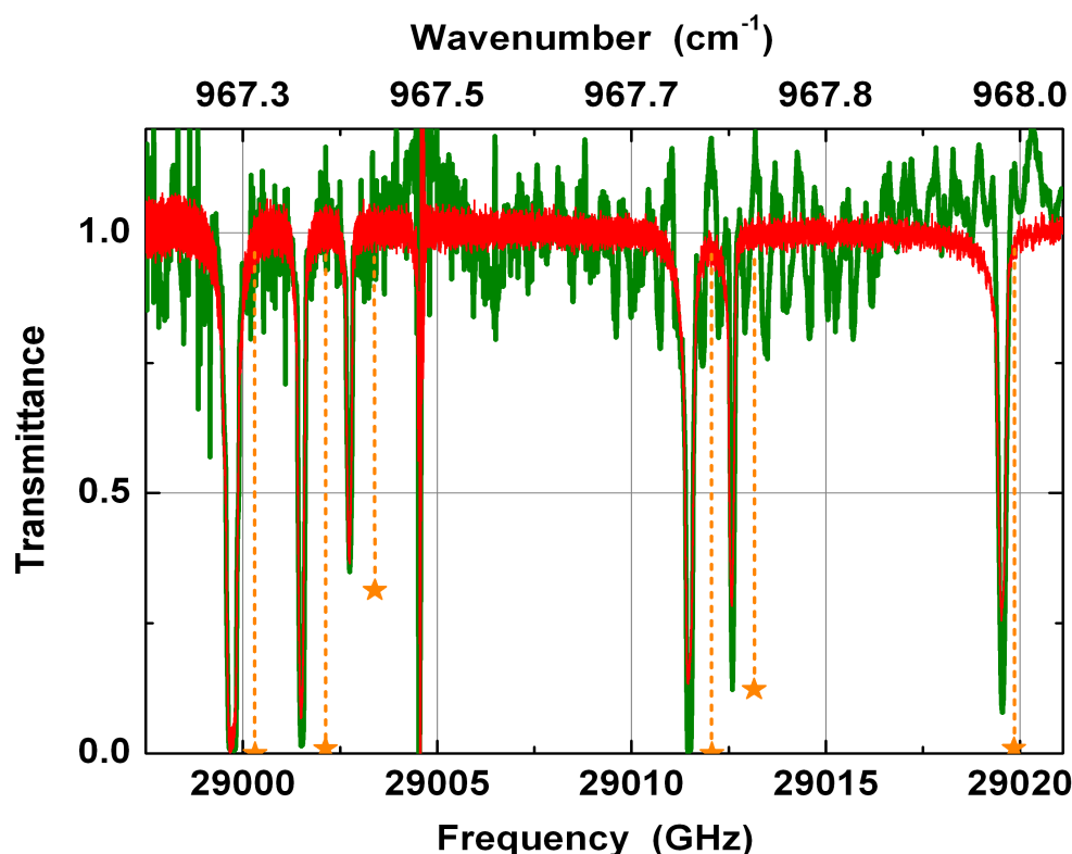
Fig. 6. Green line. NH 3 transmission spectrum obtained from the ratio between the squares of the heterodyne pulses with and without gas (the pulse with gas is the one displayed in Fig. 5(a)). Red line. NH 3 spectrum derived from the ratio between the current pulses with and without gas of Fig. 5(b). The orange stars represent the frequency and the transmission intensities of the closest NH 3 ro-vibrational transitions, based on the HITRAN database and computed with the commercial software Spectracalc ® .
