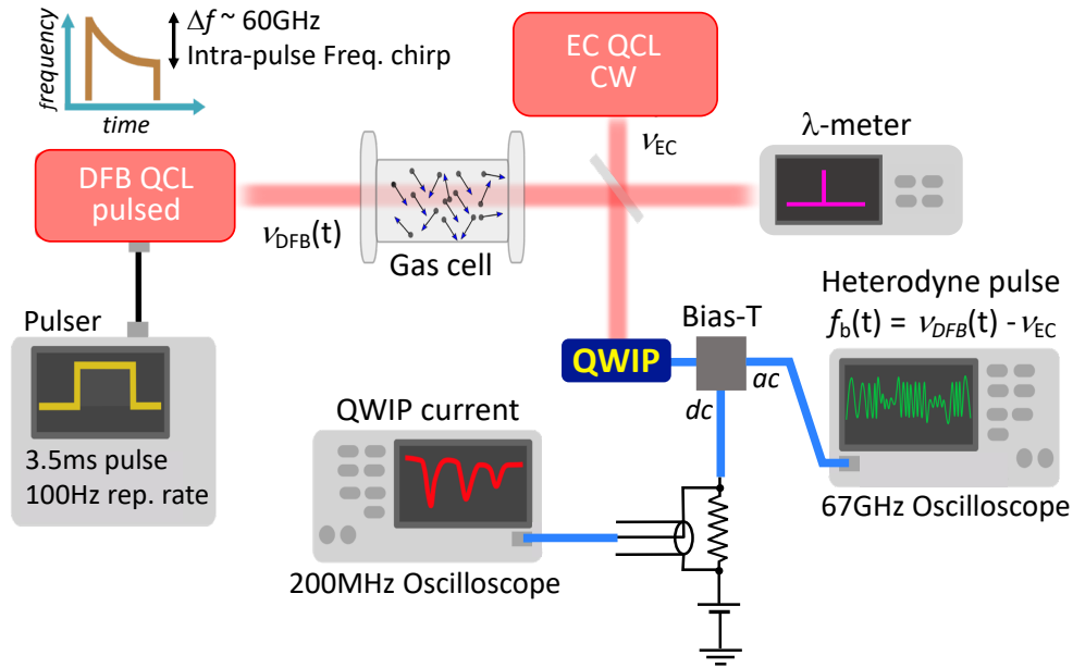
Fig. 3. Schematic of the HFCS experiment (see main text for more details). A DFB QCL, with emission frequency \nu_{DFB}(t) , is driven in pulsed mode, producing a frequency down-chirp of approximately 60GHz. Its beam is transmitted through a gas cell containing \text{NH}_3 and focused on the QWIP. A tunable EC QCL is driven in CW and provides the local oscillator for heterodyne detection. Its absolute frequency, \nu_{EC} , is monitored with a \lambda -meter. The QWIP, in series with a 34\Omega resistor, is connected to a 67GHz bias-tee and biased with a dc power supply. A 200MHz bandwidth oscilloscope is used to measure the voltage across the 34\Omega resistor, proportional to the QWIP current. The ac port of the bias-tee is connected to a 70GHz bandwidth oscilloscope, which measures in real-time the heterodyne frequency pulse, oscillating at f_b(t) = \nu_{DFB}(t) - \nu_{EC} , resulting from the mixing between the DFB and the EC QCLs.
