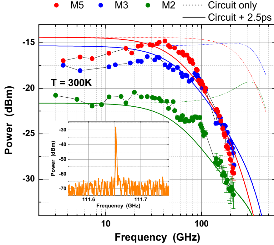
Fig. 2. (a) Room-temperature experimental frequency response of devices M5 (red dots), M3 (blue dots) and M2 (green dots) in the frequency bands 0-110GHz and 140-220GHz. The measurements are obtained at \lambda \approx 10.3\mu\text{m} by heterodyne mixing two single-mode QCLs, and the experimental values are corrected by the attenuation of the bias-tees and coplanar probes, measured with a VNA. All data was recorded without the use of any amplification stage. The incident MIR radiation is linearly polarised at 45deg with respect to the metallic wires connecting the patches, and the incident powers are 13mW and 17.5mW. The corresponding dc photocurrents are 4.1mA, 2.8mA, and 1.25mA for devices M5, M3 and M2 respectively. The dashed lines are the computed electrical frequency responses obtained from the small-signal equivalent circuit (Supplement 1, Fig. S4). The solid lines include the intrinsic ISB frequency response with a carrier capture time of 2.5ps. Inset. Example of heterodyne beatnote close to 110GHz, recorded with a spectrum analyser using the M3 photodetector. The spectrum is not corrected by the attenuation through the 110GHz probe and bias-tee.
