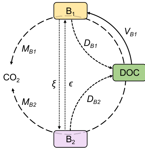
FIGURE 2 Conceptual model diagram. State variables: active biomass ( B_1 ), dormant biomass ( B_2 ), and dissolved organic carbon (DOC). Transfer functions: V_{B1} represents the growth of active biomass, M_{B1} and M_{B2} represent the maintenance of active and dormant biomass, respectively (i.e., the transformation of DOC to \text{CO}_2 by B_1 and B_2 ), D_{B1} and D_{B2} stand for the mortality of active and dormant biomass respectively, \xi is the de-activation of active to dormant biomass, and \epsilon is the activation of dormant biomass to active biomass.
