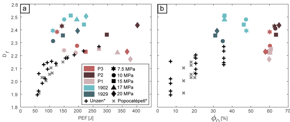
Fig. 11 The fractal dimension of experimental results on materials from Mt. Pelée from this study, together with results for Popocatépetl (Mexico) and Unzen (Japan) materials (*) from Perugini and Kueppers (2012), compared with potential energy of fragmentation (a) and open porosity (b)
