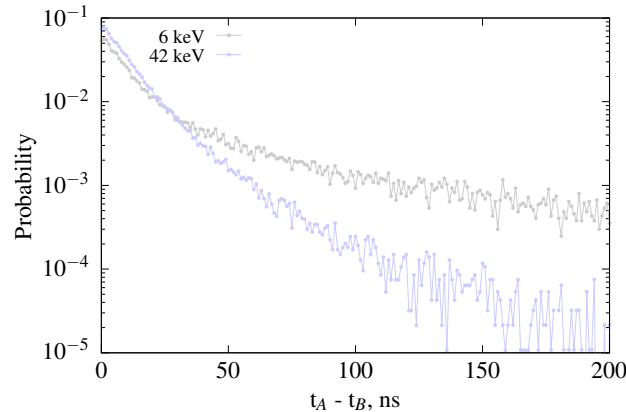
Figure 11. Time interval distribution of photon produces by YAG(Ce) for an energy of 42 keV and 6 keV.
