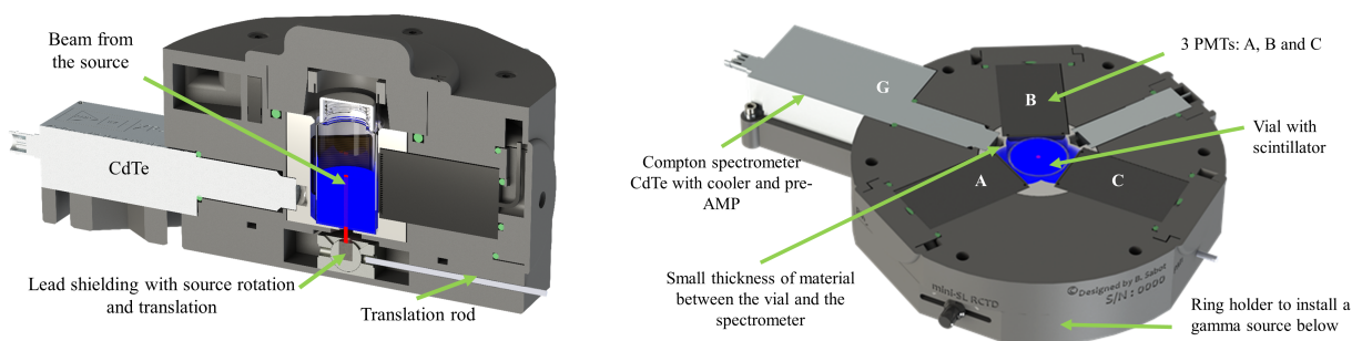
Figure 13. Left: Vertical cut of the system – the red line represents the beam of the source, the bright blue correspond to the size of scintillator ; Right: Horizontal cut of the system at the position of the CdTe detector.
