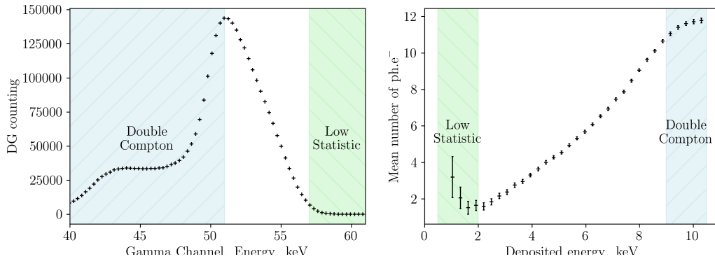
Figure 17. On the left, the obtained compton spectra in coincidence with D channel, on the right the extracted non-linearity curve. The boundaries are represented in colors on the pictures to illustrate our current limitations.
