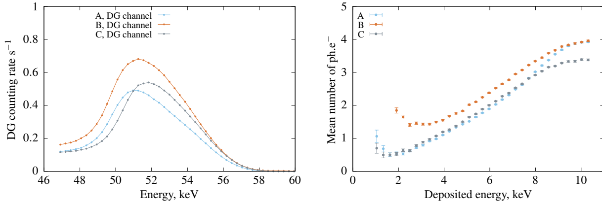
Figure 5. Left: Compton spectrum in the \gamma channel for events in coincidence with D. Right: Non-linearity curves showing the evolution of the mean number of photo-electrons as a function of the electron energy for the 3 plastic scintillators.
