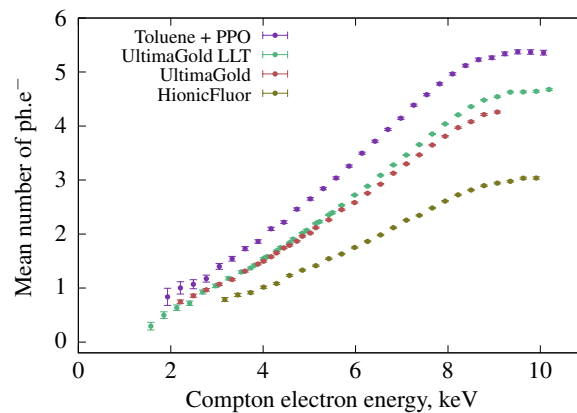
Figure 1. Relative light output of Ultima Gold, Ultima Gold LLT, toluene + PPO and HionicFluor cocktails.
