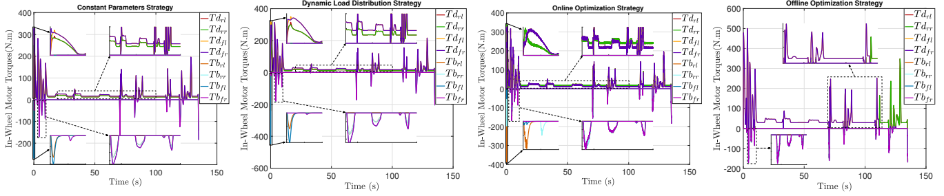
Fig. 21: In-Wheel Motors Driving and Braking Torques of the Proposed Strategies: Decentralized Approach - Sc1 (b)
