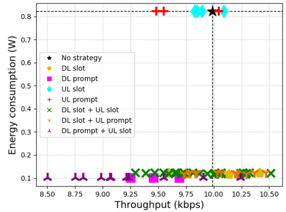
Figure 4: Case study 2. Performance of the energy-saving strategies for various configurations of their parameters.
