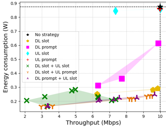
Figure 3: Case study 1. Performance of the energy-saving strategies for various configurations of their parameters.
