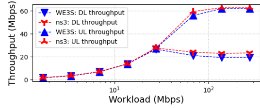
Figure 2: Accuracy of WE3S at reproducing the aggregated downstream and upstream throughput in a WLAN with 1 AP and 3 STAs.
