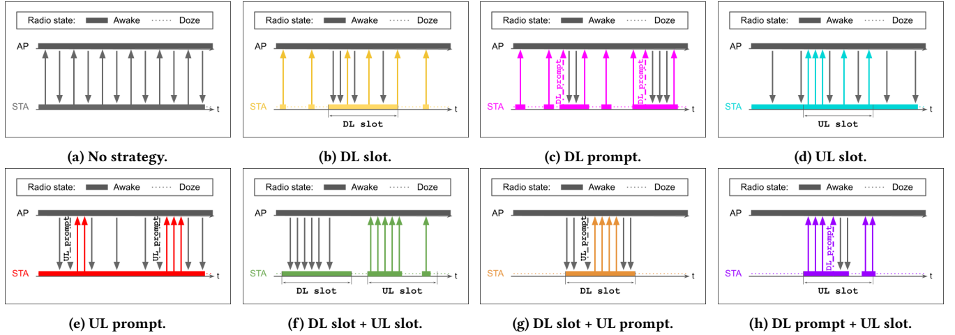
Figure 1: Possible strategies to save energy at the MAC layer of 802.11.
