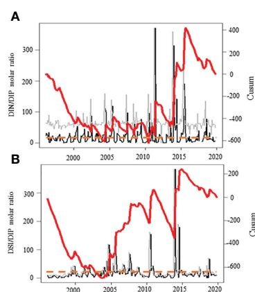
FIGURE 2 Temporal variations of the nutrient molar ratios (A: DIN/DIP, B: DSI/DIP, [ \mu M:\mu M ], with DIN and DIP as dissolved inorganic nitrogen [i.e., the sum of nitrates, nitrites and ammonium]) and phosphorus in coastal waters of the eastern English Channel over the period 1996–2019. Black line: monthly raw time-series. Grey line: seasonally adjusted, and red thick line: Cusum. Right axes are for seasonally adjusted and Cusum. Orange dashed line: the Redfield and Brzezinski nutrient molar ratios (Redfield 1963; Brzezinski 1985).
