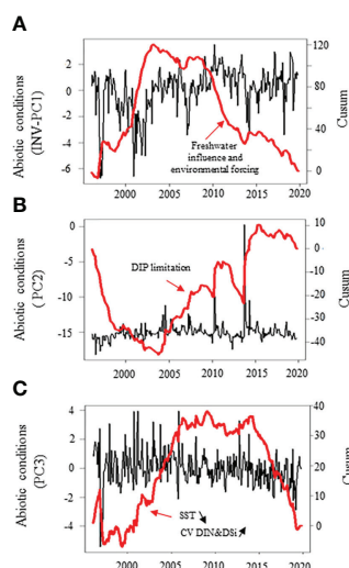
FIGURE 4 Temporal variations of the abiotic conditions (mean and variability) in coastal waters of the eastern English Channel over the period 1996–2019. (A) Principal component 1 (INV-PC1); (B) Principal component 2 (PC2); and (C) Principal component 3 (PC3, see Figure S1 for PCA details). Black line: monthly seasonally adjusted ones. Red thick line: Cusum. Right axes are for Cusum. Note that PCs values in (A) have been inverted for ease of reading with next results (Figure 5).
