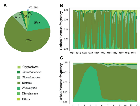
FIGURE 3 (A) Whole phytoplankton composition (carbon biomass frequency), and its (B) temporal and (C) average seasonal variations, respectively, in coastal waters of the eastern English Channel over the period 2009–2019.
