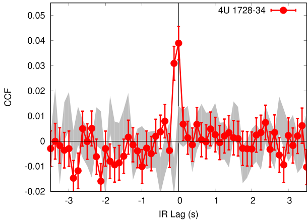
Figure 3. CCF computed between XMM-Newton and HAWKI-I for 4U 1728–34 (red points) and the comparison star (grey curve).
